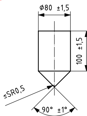
Figure 7 — Test cone
