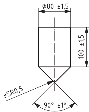
Figure 7 — Test cone
