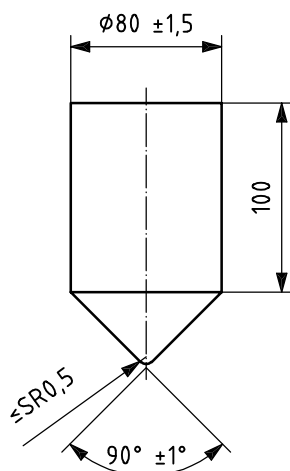
Figure 3 — Test cone
