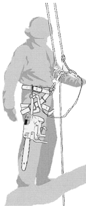
Figure B.1 — Example of attachment of tree service chain-saw to operator's harness
