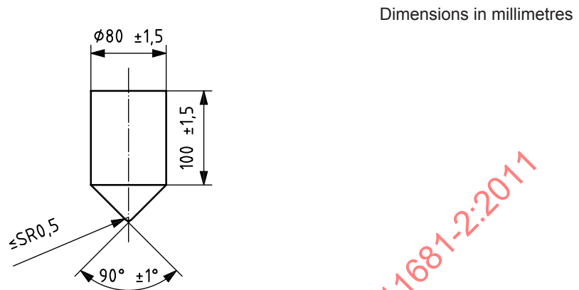
Figure 3 — Test cone
