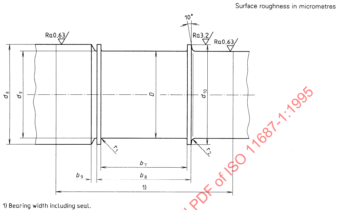
Figure 3 — Shaft design for non-locating (free) bearing (thrust bearing part Q)
