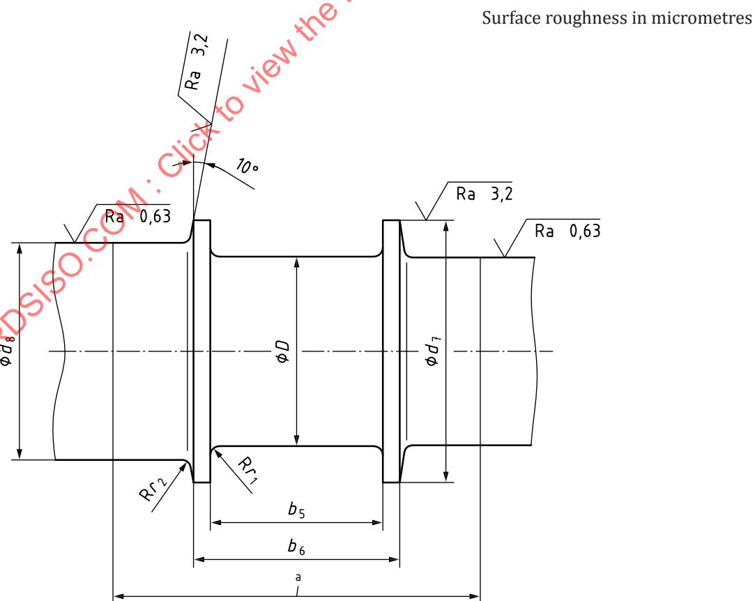
Figure 3 — Shaft design for non-locating (free) bearing (thrust bearing part Q)
