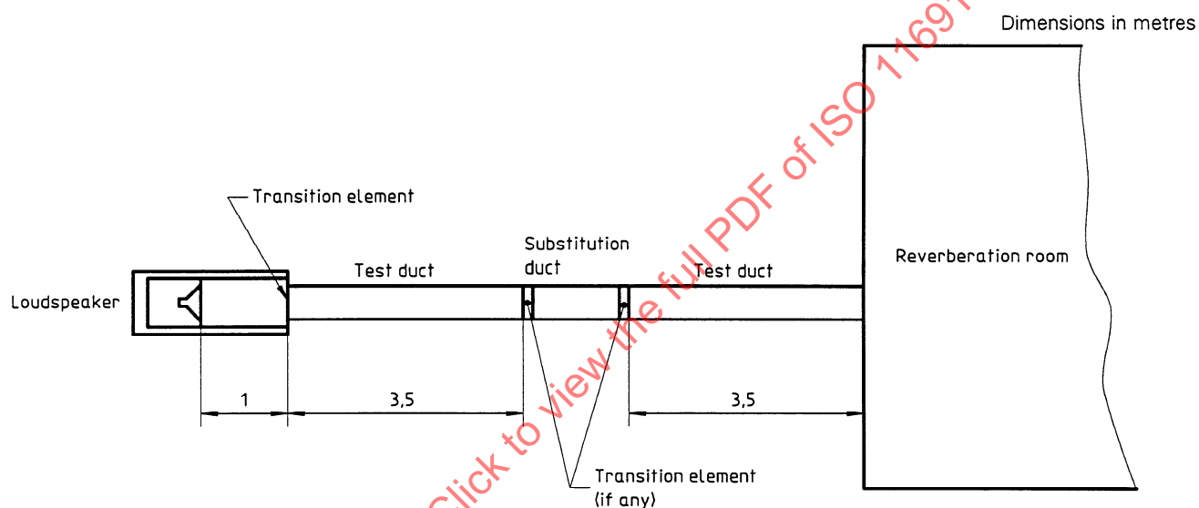
Figure 1 — Test facility
