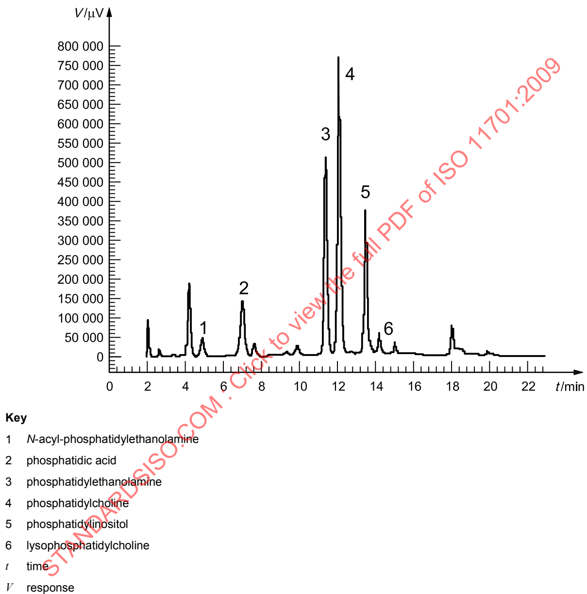
Figure A.1 — HPLC chromatogram of phospholipids of crude native soya lecithin
