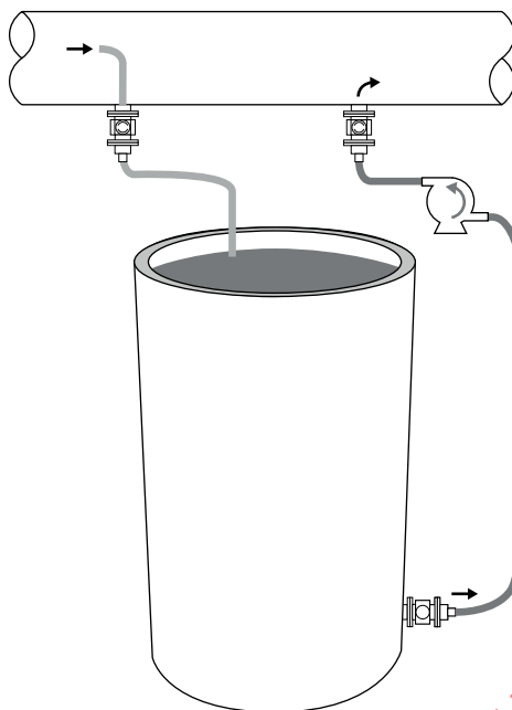
Figure A.3 — Open system with filtrate pumped back to ballast discharge line via closed loop configuration
