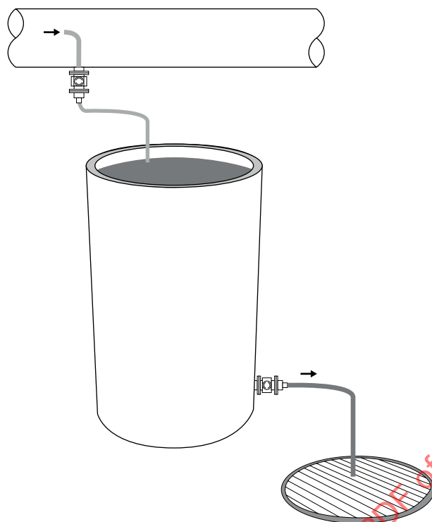
Figure A.1 — Open system with disposal of filtrate to ship drain via open loop configuration
