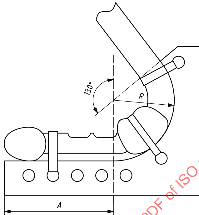
Figure C.3 — Example of strapping a laryngeal tube-type supralaryngeal airway to the template
