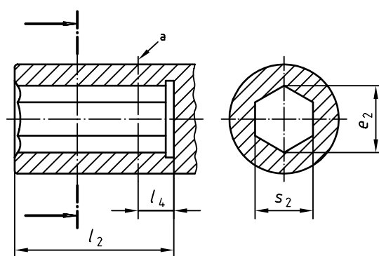
Figure 6 — Female hexagon form F
