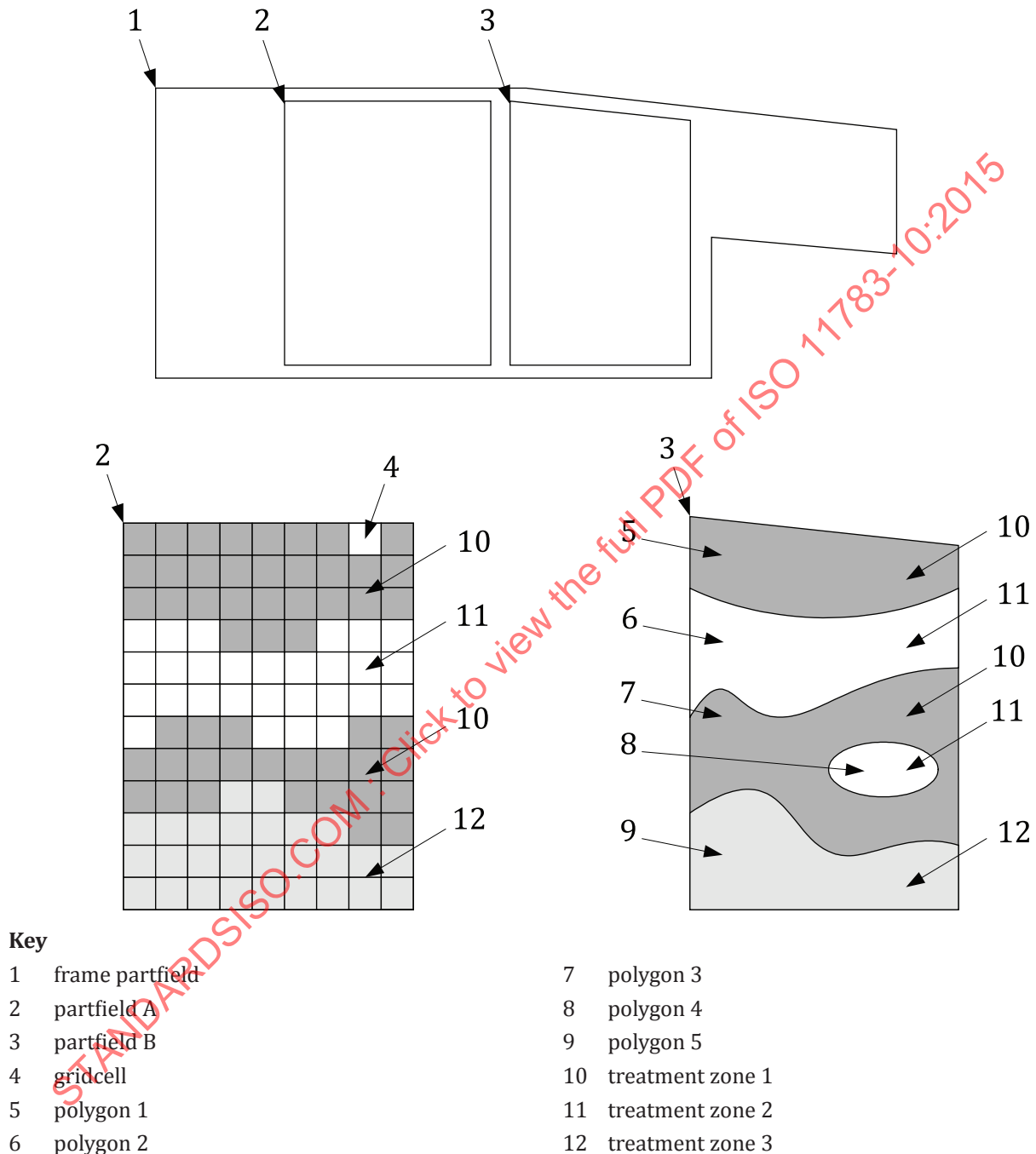
Figure 3 — Frame partfield, partfield, gridcell, polygon, treatment zone relationship
