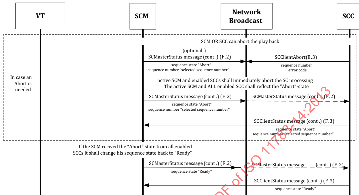
Figure 12 — Abort message flow diagram
