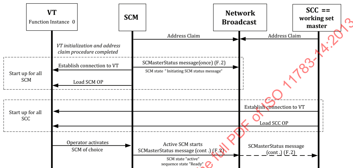
Figure 6 — Initialization message flow diagram for SCC as working set master
