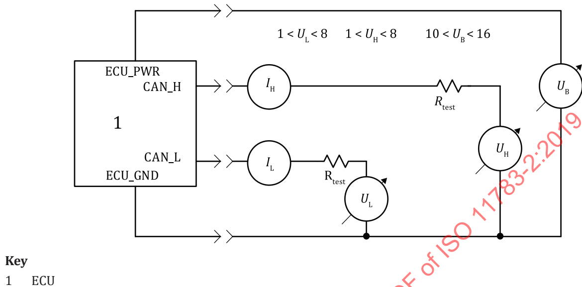
Figure 40 — Measurement of V_{CAN\_H} and V_{CAN\_L} while the ECU sends a dominant bit
