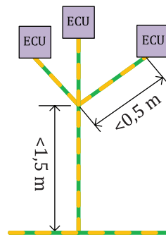
Figure 13 — Compound stub
