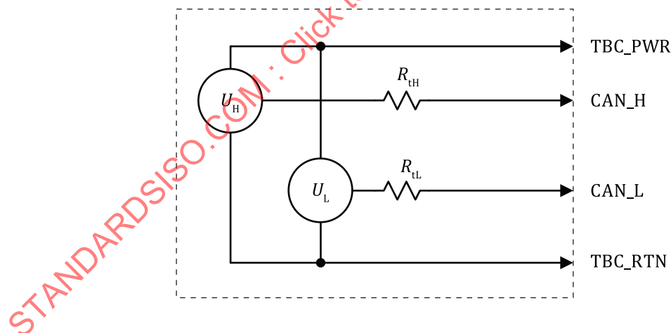
Figure 17 — Equivalent terminating bias circuit (TBC)
