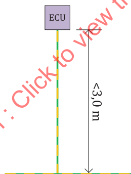
Figure 11 — Simple stub
