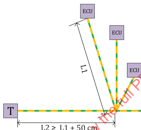
Figure 15 — Multiple splice
