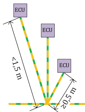
Figure 15 — Multiple splice
