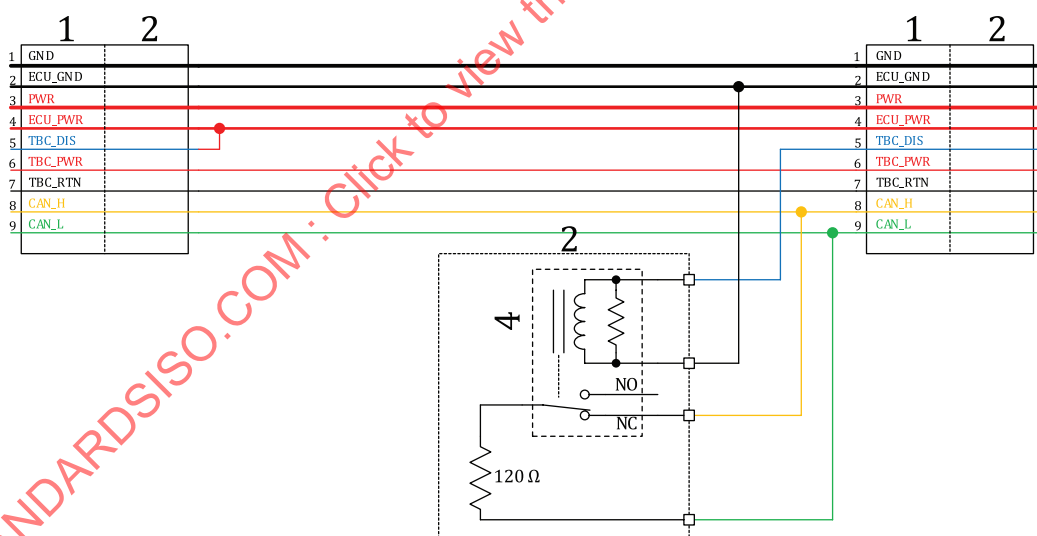
Figure 27 — TPPL implement, daisy chain (single fuse)
