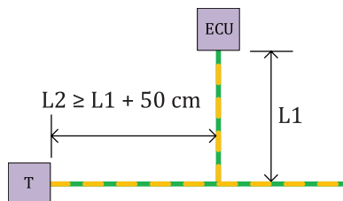
Figure 11 — Simple stub
