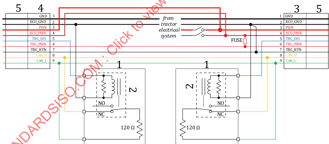
Figure 23 — TPPL tractor with rear TPPL Breakaway Connector
