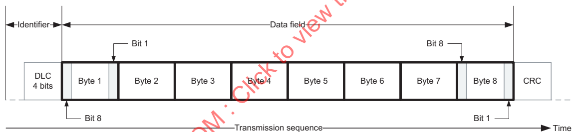
Figure 3 — CAN data field
