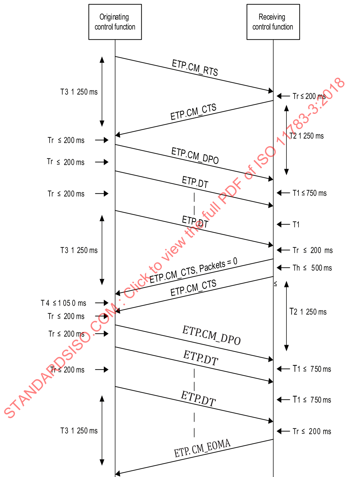
Figure 8 — Extended transport message sequence
