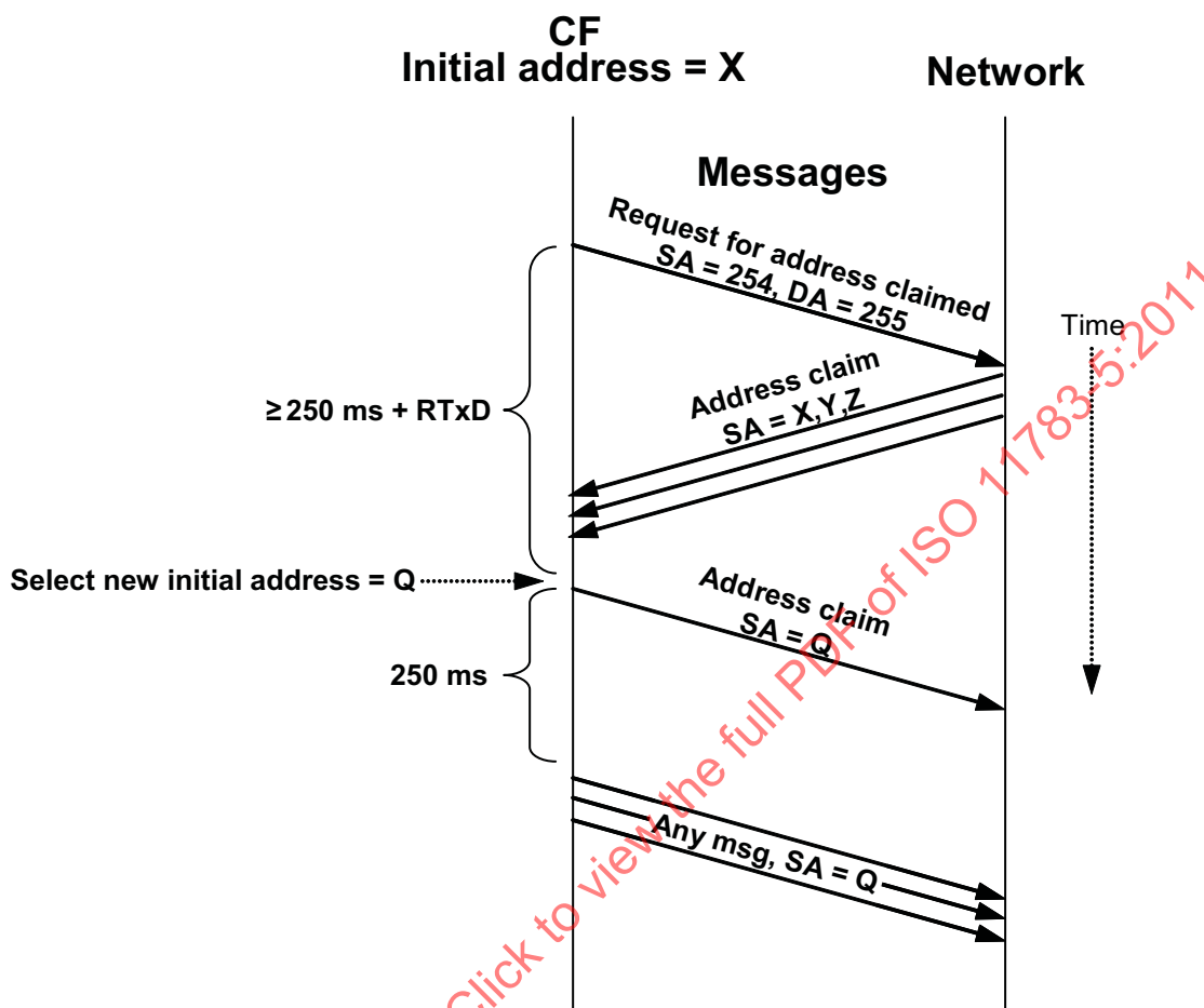
Figure 5 — Resolving initial addresses without contention
