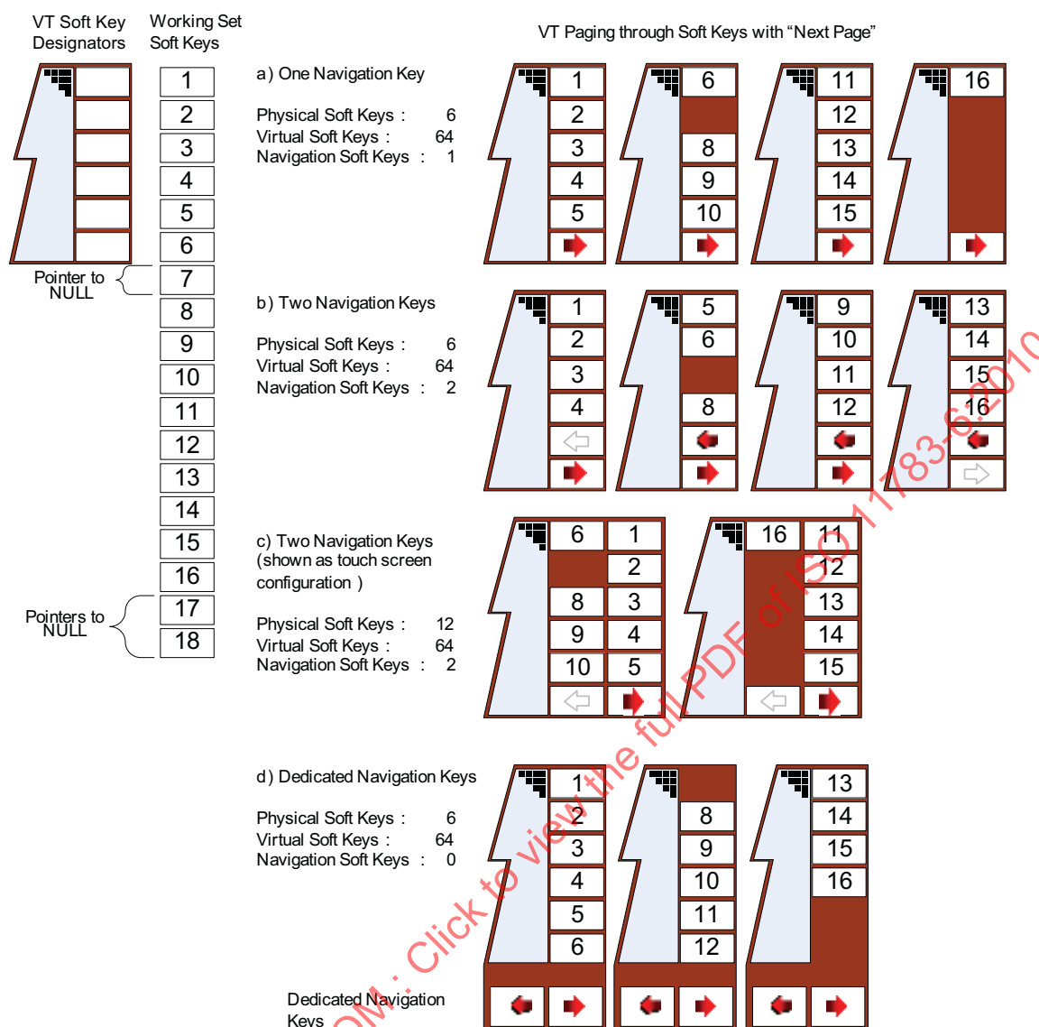
Figure 4 — VT virtual Soft Key paging
