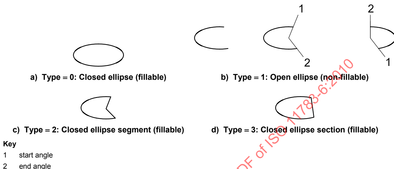
Figure B.6 — Ellipse object
