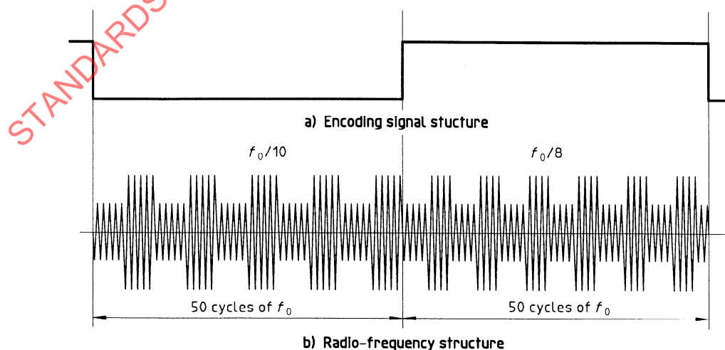
Figure A.1 — Signal structures of binary 0 of Destron (FECAVA version)
