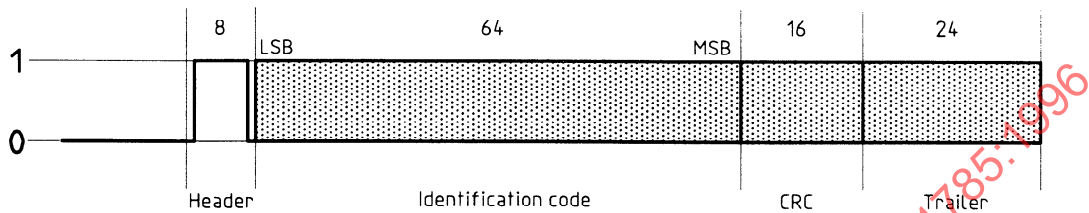
Figure 5 — Structure of the HDX identification telegram
