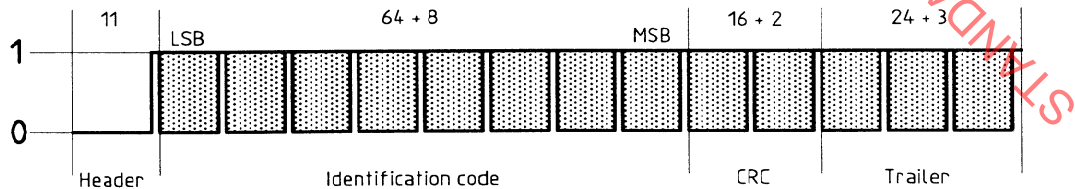
Figure 2 — Structure of the FDX identification telegram
