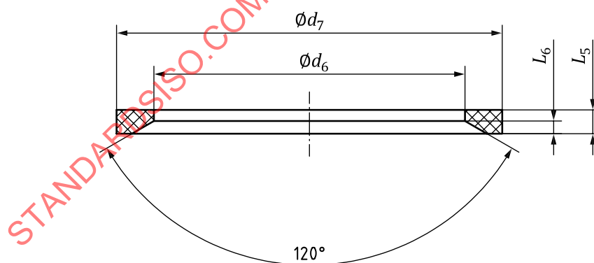
Figure 2 — Elastomeric seal for use with ISO 1179-2 heavy-duty (S series) and light-duty (L series) stud ends
