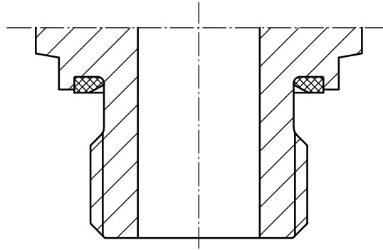
Figure 3 — Correct assembly of elastomeric seal on stud end
