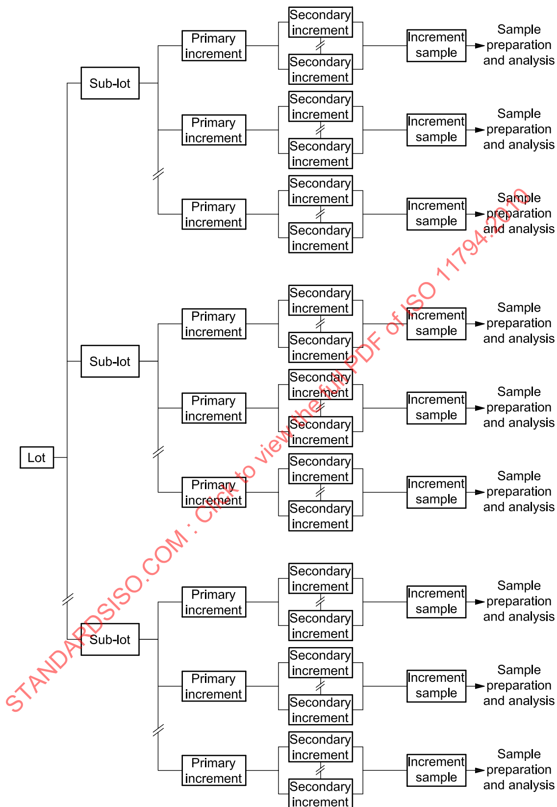
Figure 5 — Example of a sampling plan with each increment analysed separately
