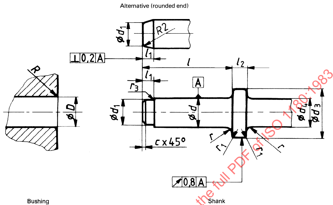
Figure 1 — Coal pick shanks and corresponding chuck bushings
