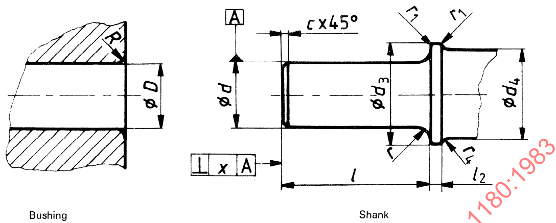
Figure 5 — Rivet snap shanks and corresponding chuck bushings, parallel
