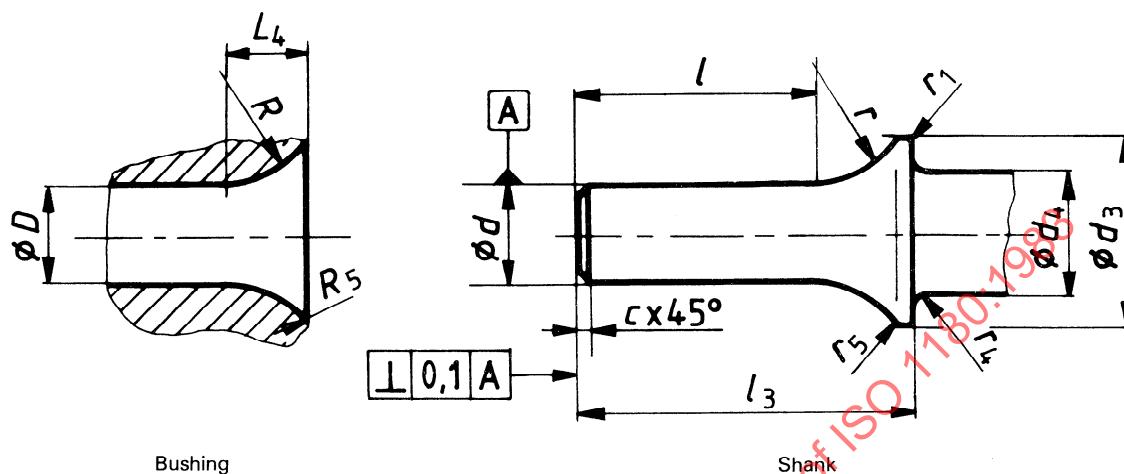
Bushings
