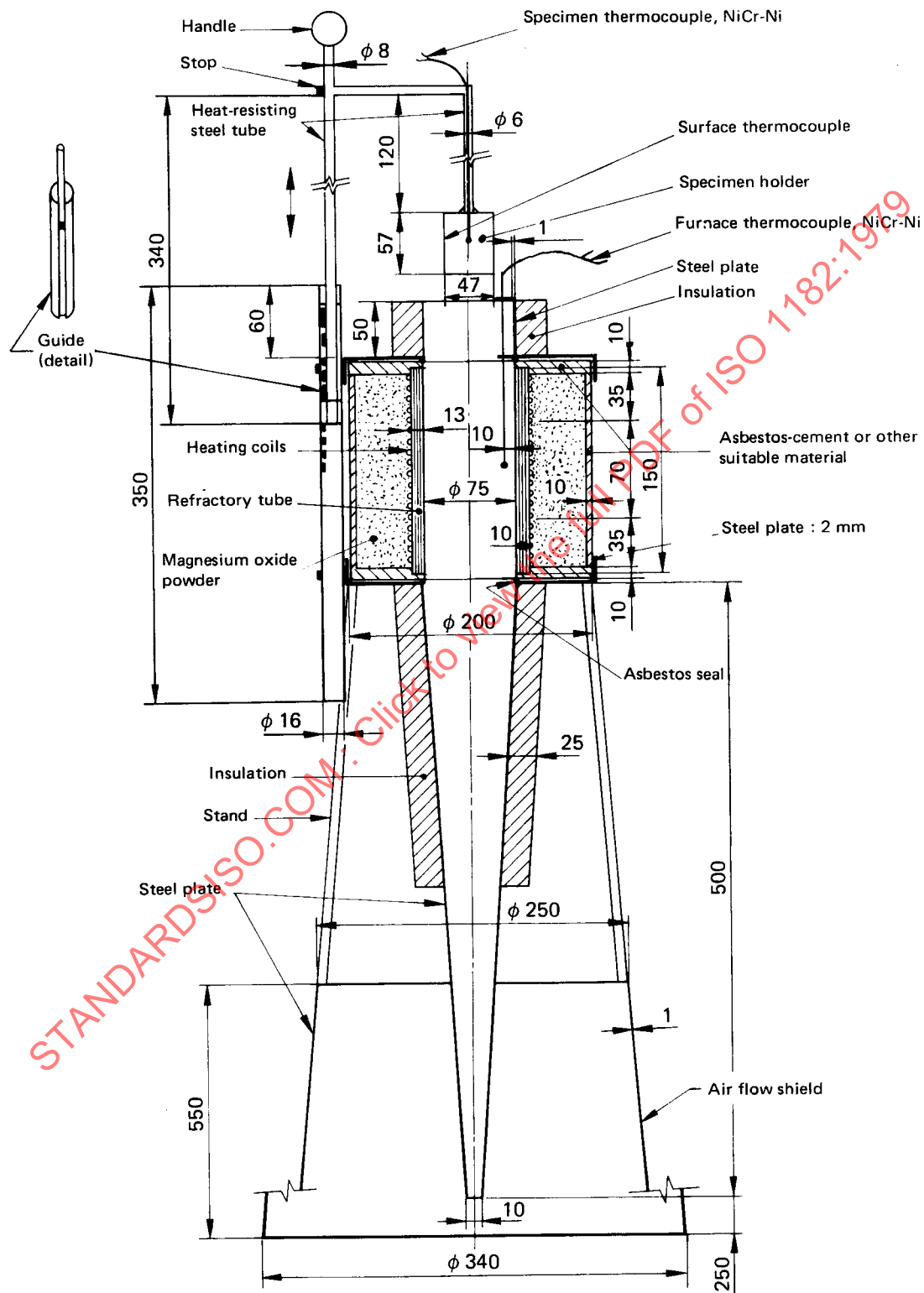
FIGURE 1 — Non-combustibility test apparatus — General arrangement
