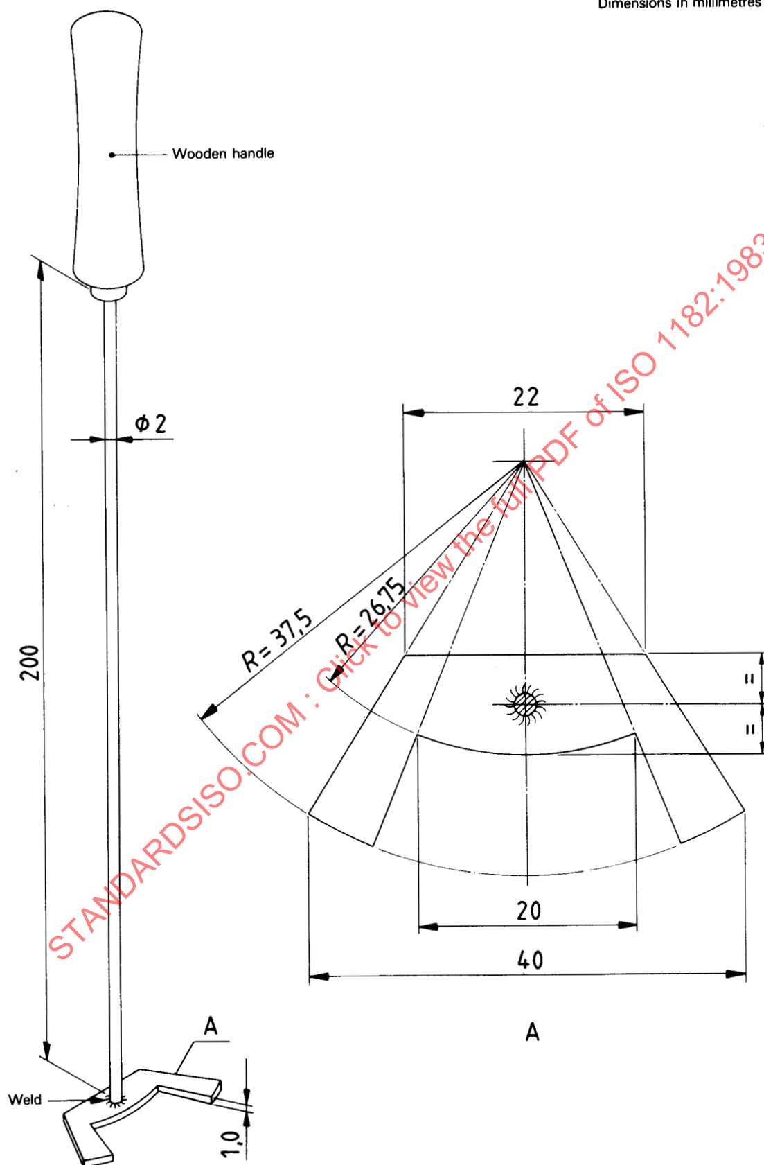
Figure 4 — Locating guide
