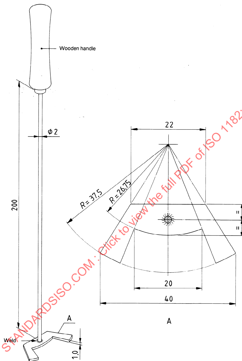
Figure 4 — Locating guide
