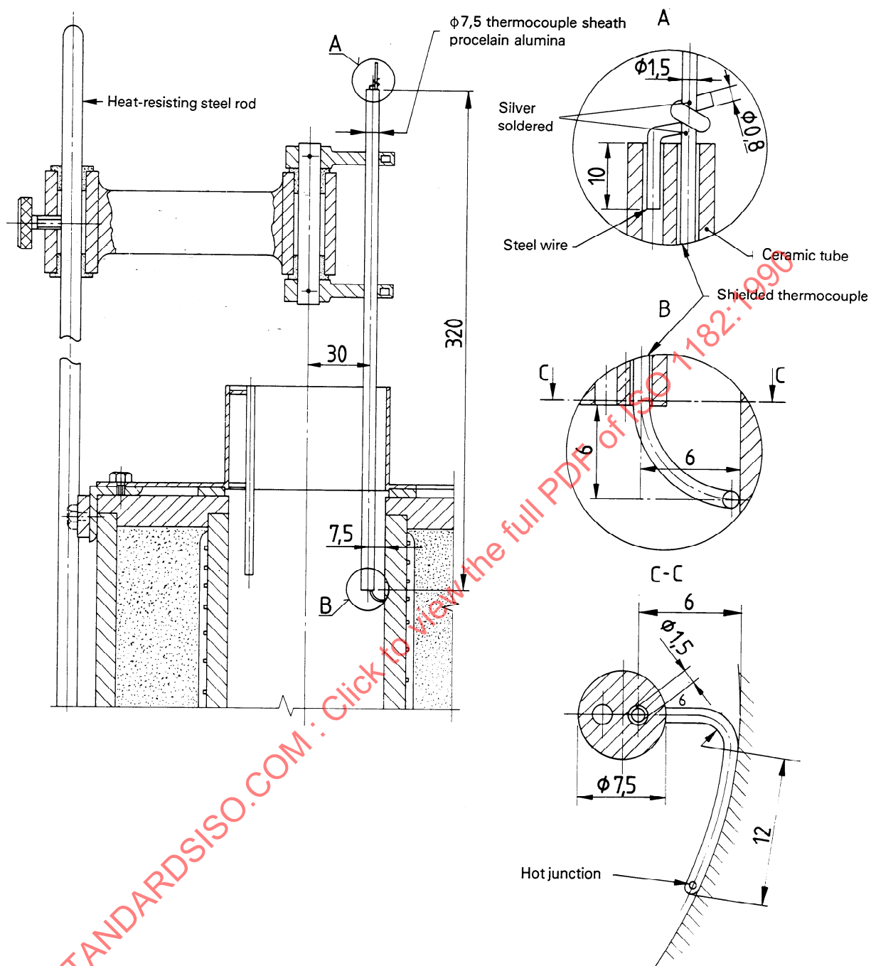
Figure 7 — Thermocouple scanning device
