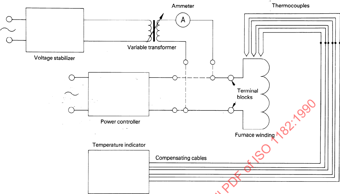
Figure 6 — Layout of apparatus and additional equipment
