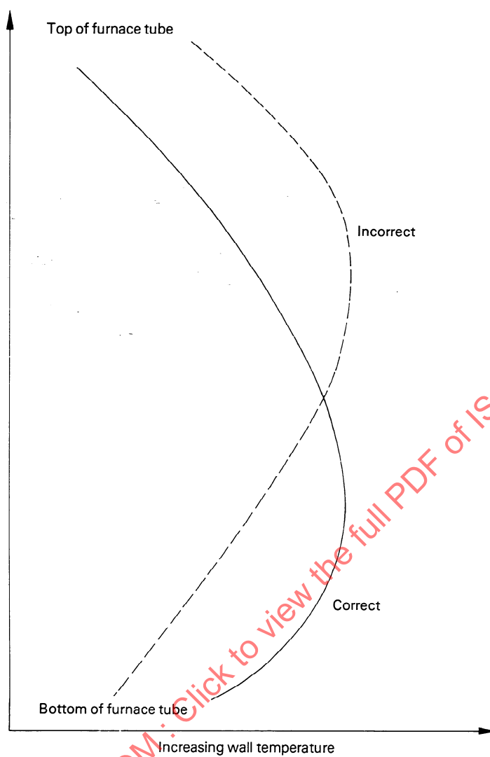
Figure 8 — Furnace wall temperature profile
