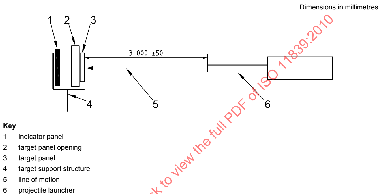
Figure 1 — Illustrative arrangement of test equipment
