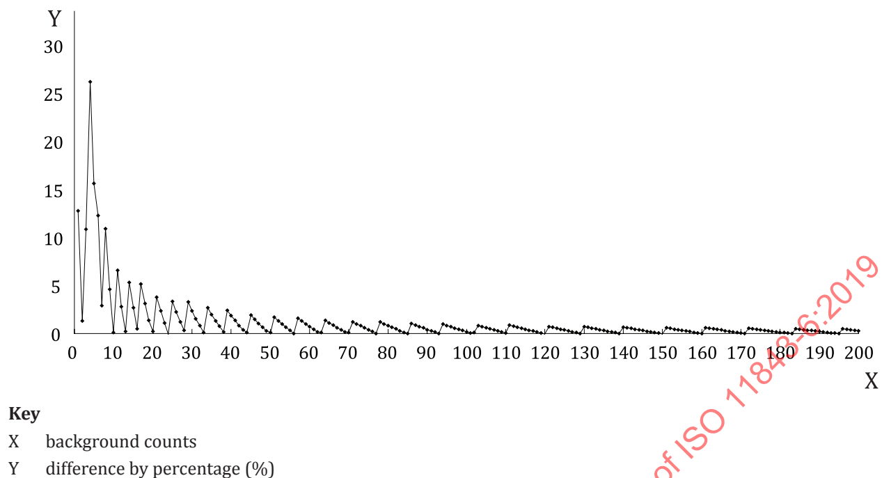
Figure C.1 — The variation in the percent difference between the Poisson distribution and the normal approximation with the background value
