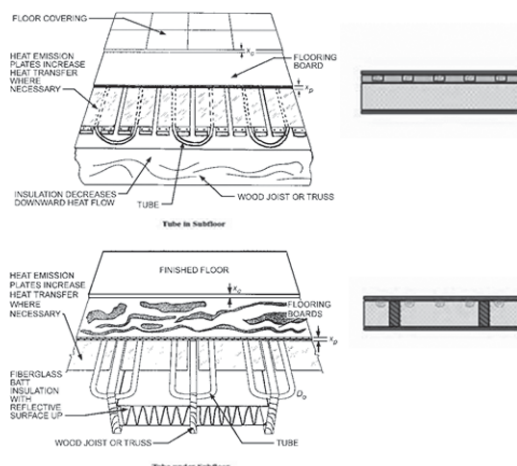
Figure 6 — Pipes in wooden constructions, TYPE G
