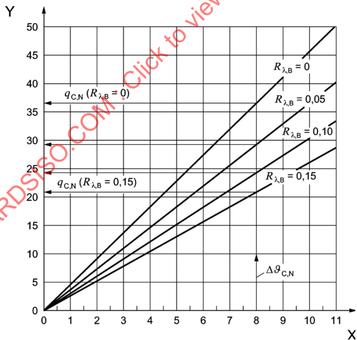
Figure A.5 — Field of characteristic curves of a heating system
