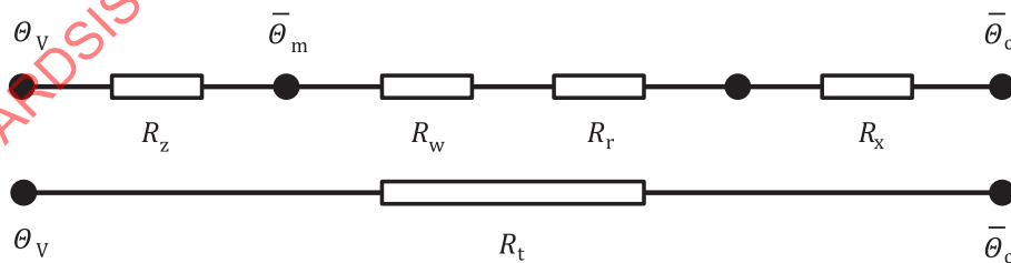
Figure B.2 — Overall resistance network
