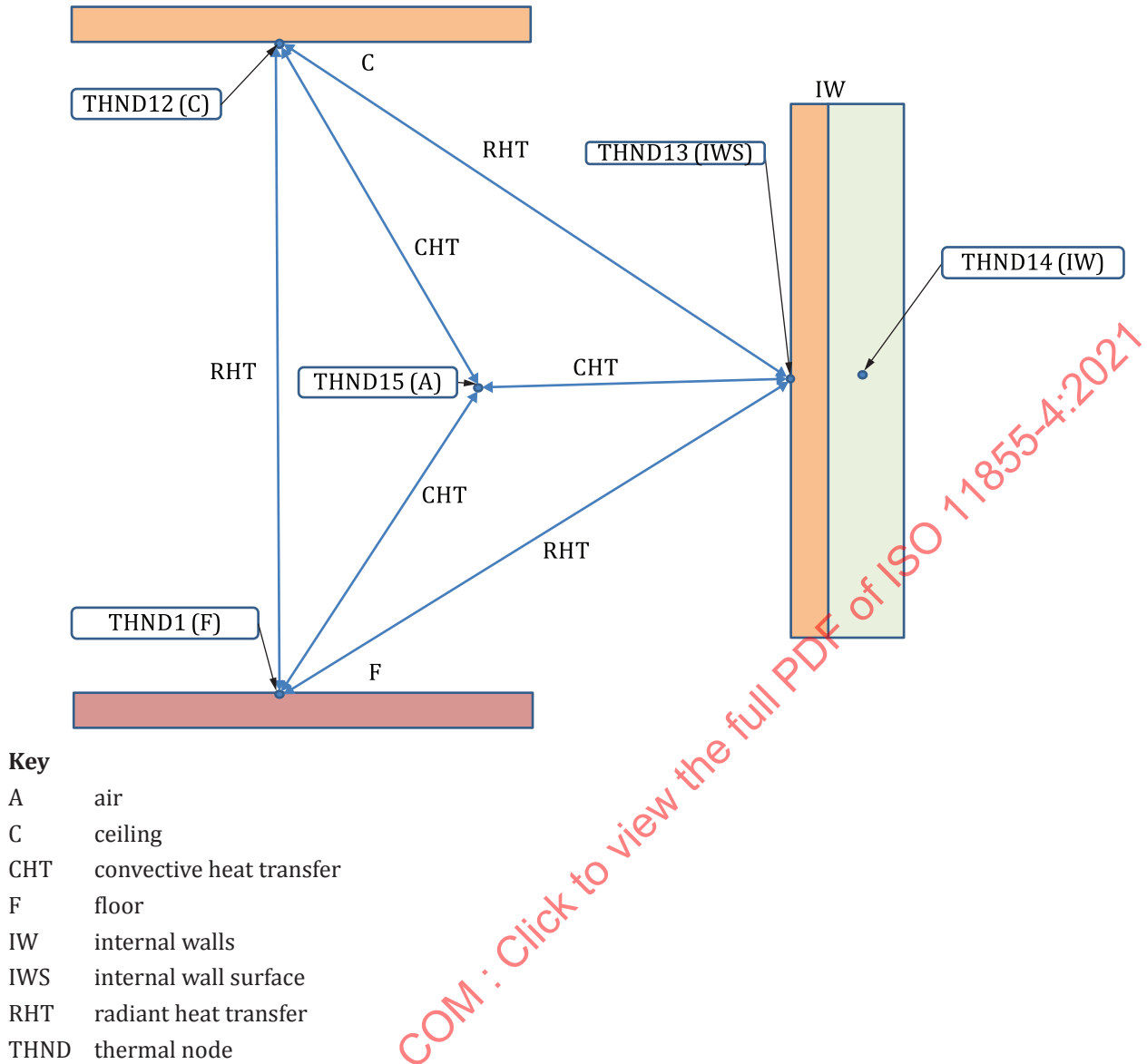
Figure B.2 — Example of thermal nodes representing the room and correlated heat transfer connections
