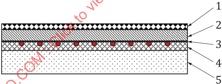
Figure A.1 — Construction of typical floor heating systems — Wet system (type A or C)
