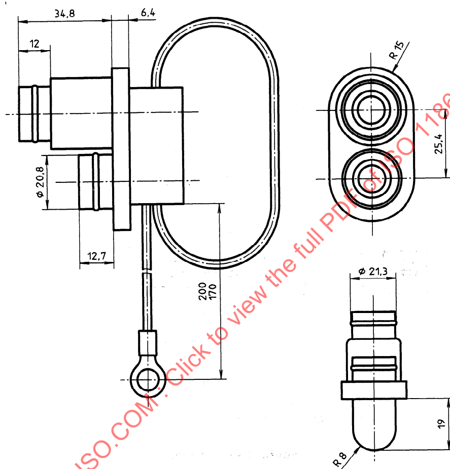
Figure 4 — Cover assembly
