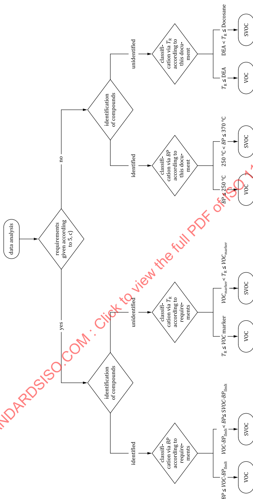
Figure 4 — Scheme for classification of compounds
