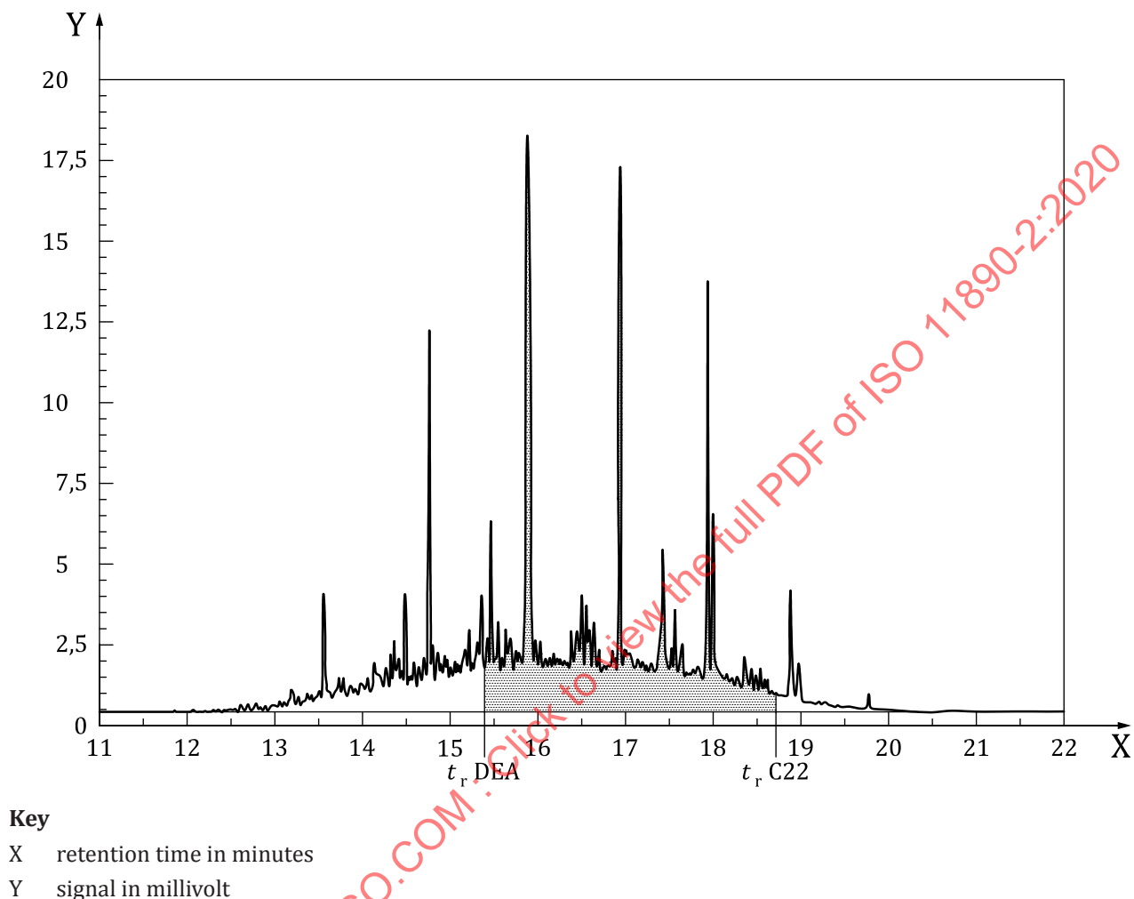
Figure 3 — Illustration of appropriate integration method for complex mixtures of chemical homologues that cannot be resolved
