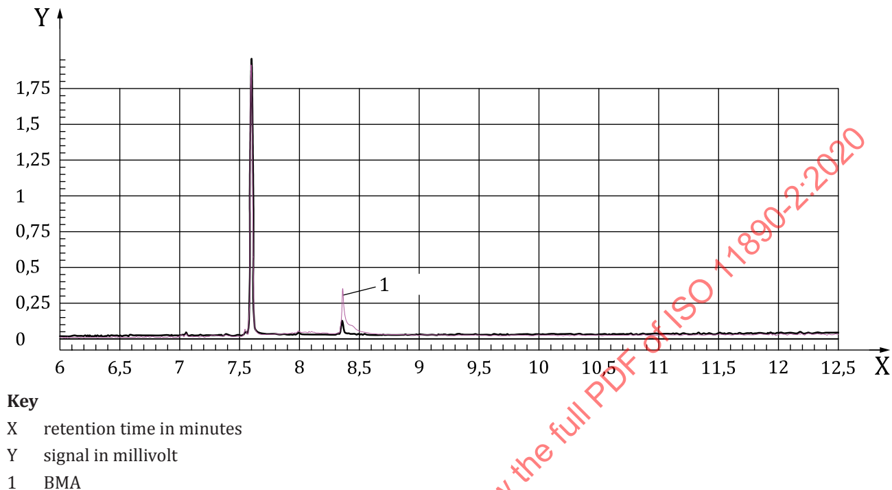
Figure B.2 — Overlay chromatogram of a poly-methacrylate injected at 175 °C (black) and 250 °C (pink)
