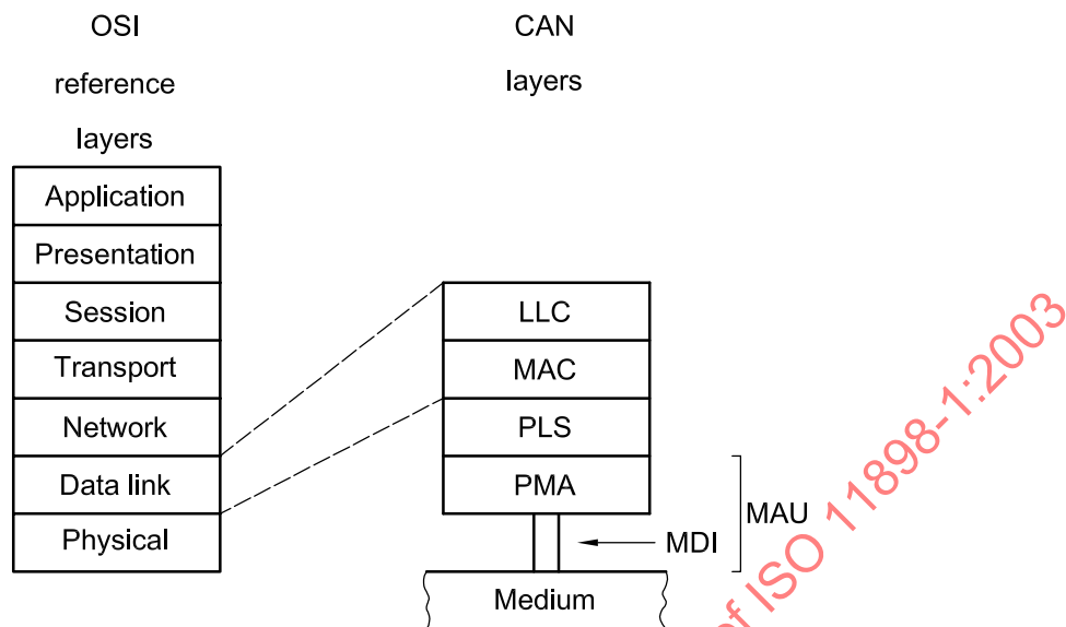
Figure 12 — Model of PL architecture
