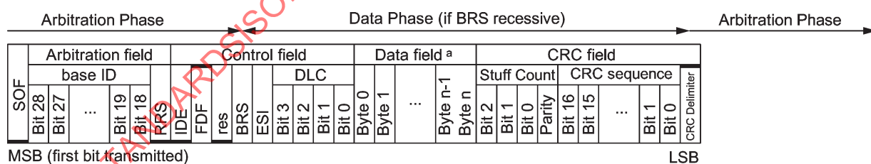
Figure 12 — Order of bit transmission in Classical Base Frame Format, up to 8 data bytes
