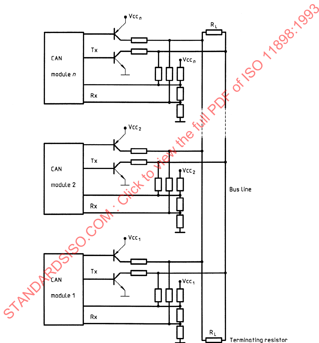
Figure 15 — Suggested electrical interconnection
