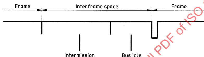
Figure 9 — Interframe space for nodes which are not "error-passive" or have been receiver of previous frame
