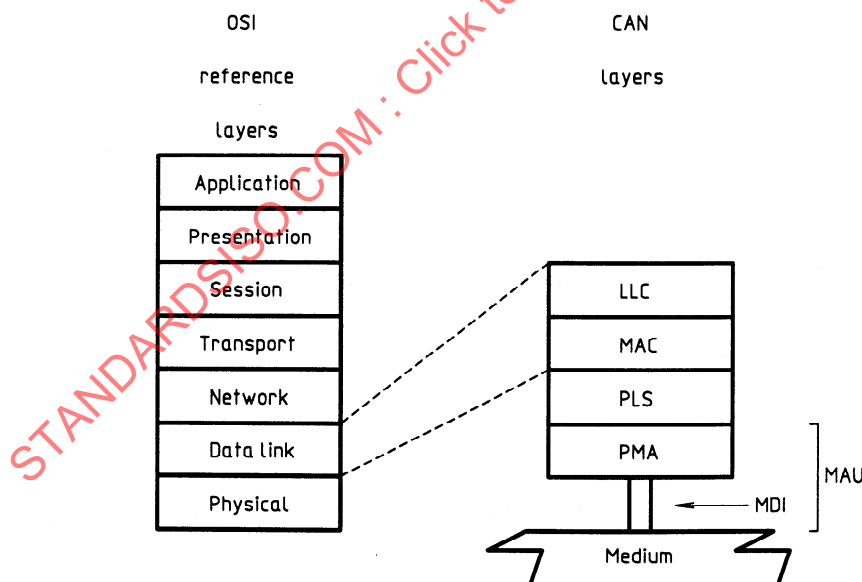
Figure 13 — Model of physical layer architecture
