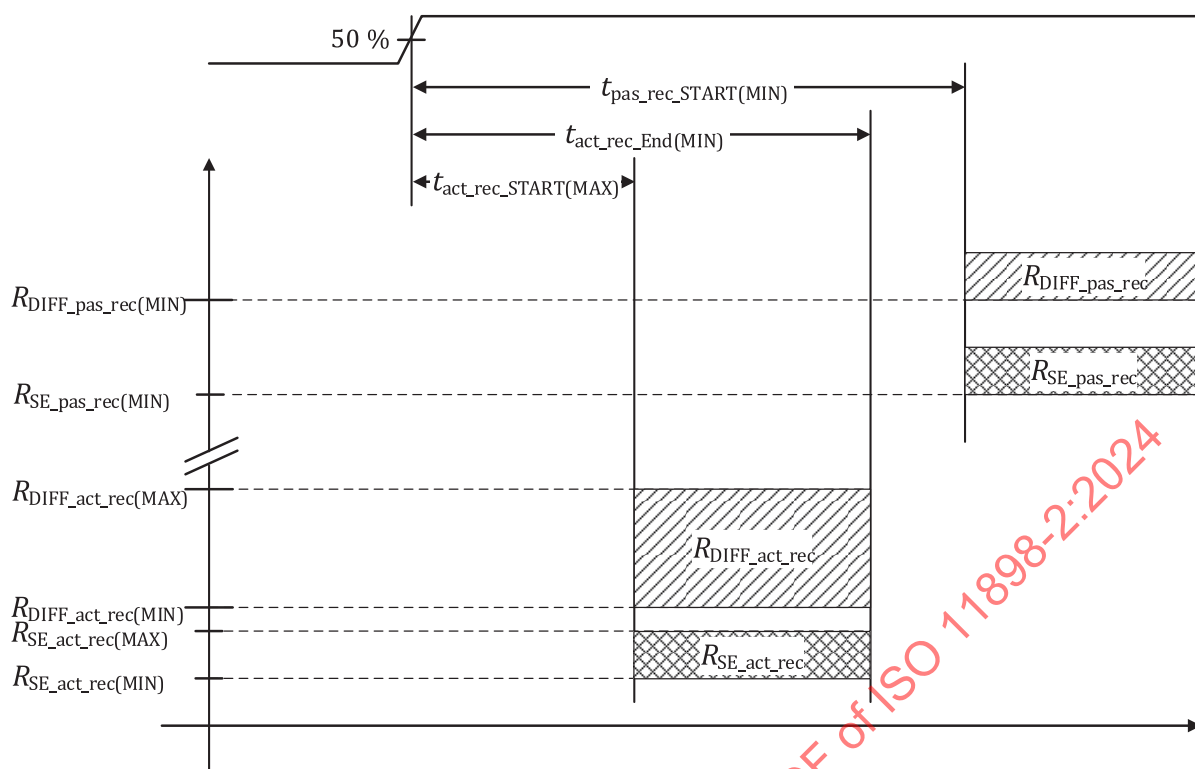
Figure 6 — SIC timing definitions
