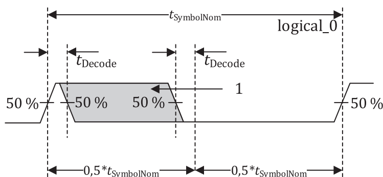
a) Transmitting PMA worst-case level_0 PWM symbol to be decoded
