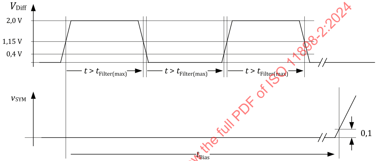
Figure 15 — Test signal definition for bias reaction time measurement
