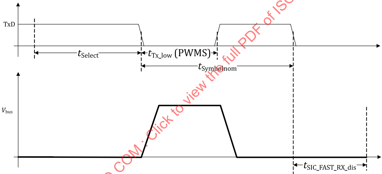
Figure A.14 — PMA implementation timing diagram, SIC mode time after FAST RX detection
