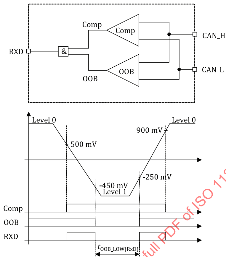
Figure A.4 — OOB and comparator signals when RXD is in SIC mode
