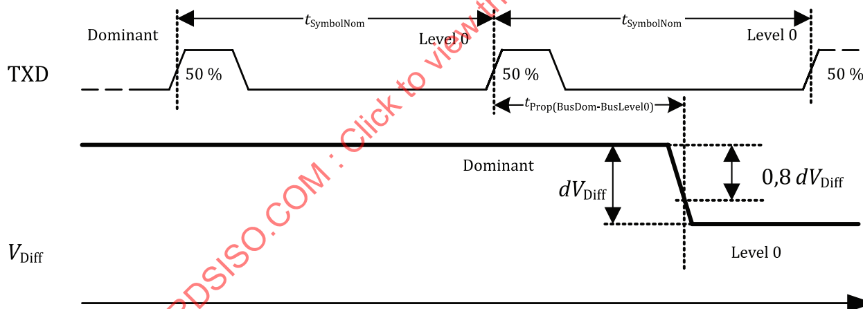
Figure A.12 — PMA implementation timing diagram, transition SIC mode to FAST TX mode, PWM driven
