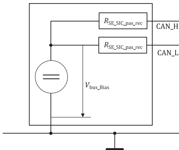
Figure 4 — Illustration of HS-PMA internal differential input resistance
