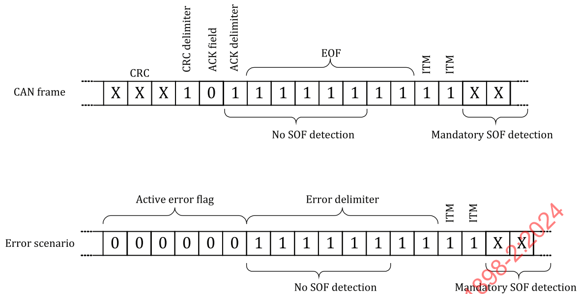
Figure 11 — Mandatory SOF detection after classical CAN frames and error scenarios
