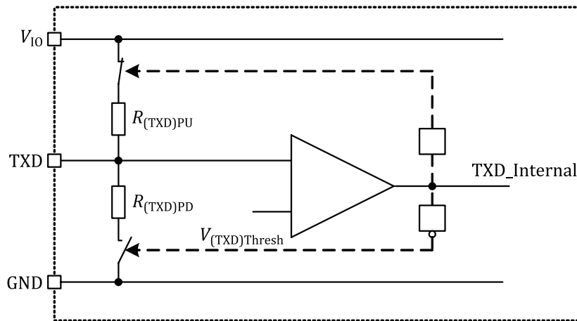
Figure A.8 — TXD input circuitry
