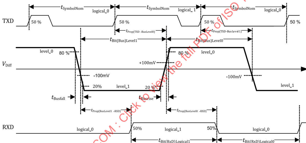
a) Overview timing diagram in FAST TX mode
