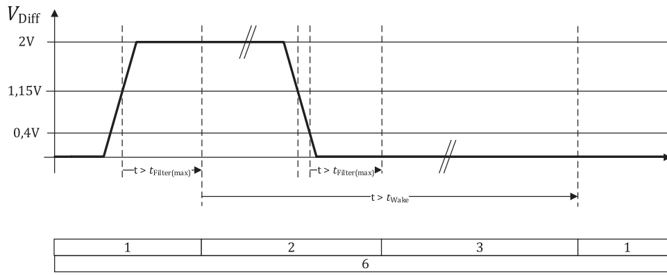
c) Incorrect wake-up pattern, recessive phase longer than t_{Wake}
