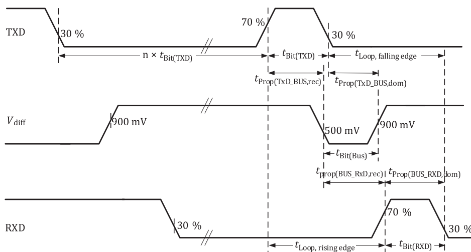
Figure A.9 — PMA implementation timing diagram, during SIC mode
