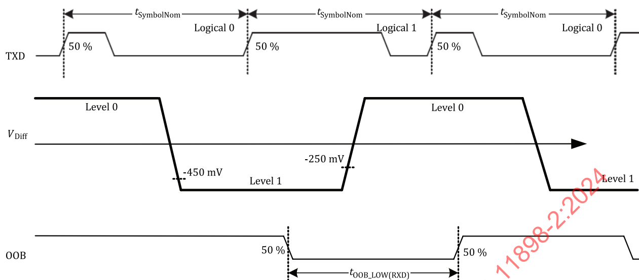
Figure A.11 — PMA OOB implementation timing diagram, during SIC mode, PWM driven
