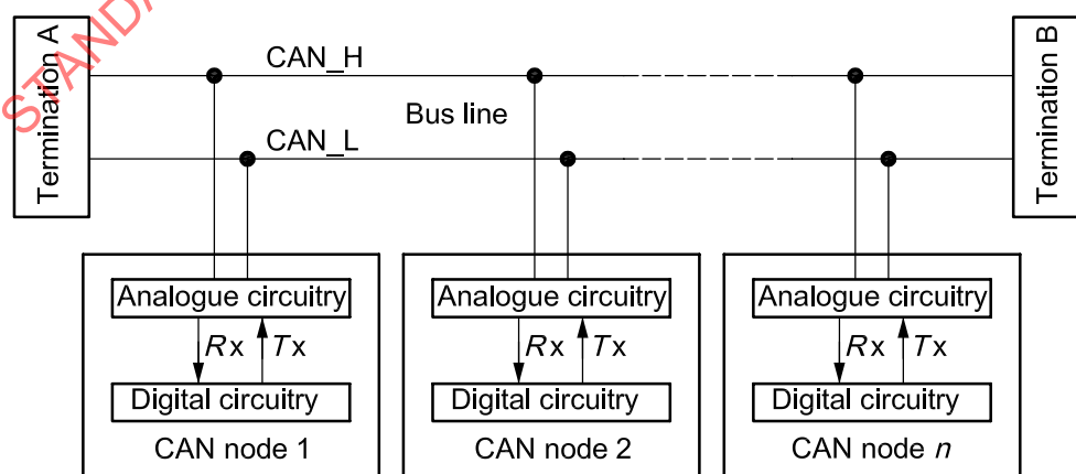
Figure 1 — Suggested electrical interconnection
