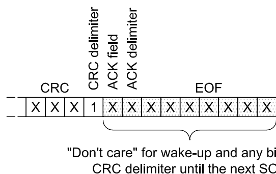
Figure 6 — “Don’t care” bits for frame decoding
