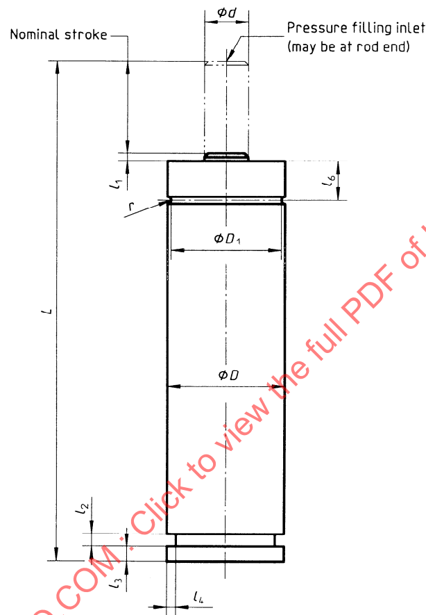
Figure 2 — Gas springs of nominal force between 1 000 N and 2 500 N
