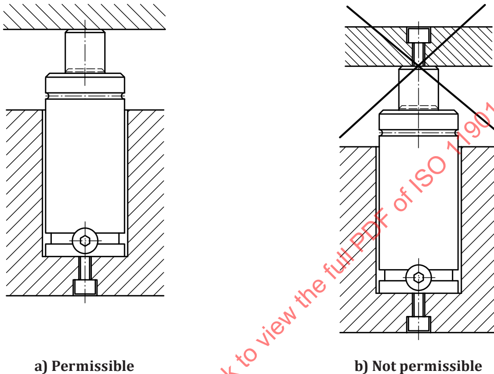
Figure A.14 — Alternative mounting - bolted to the spring base
