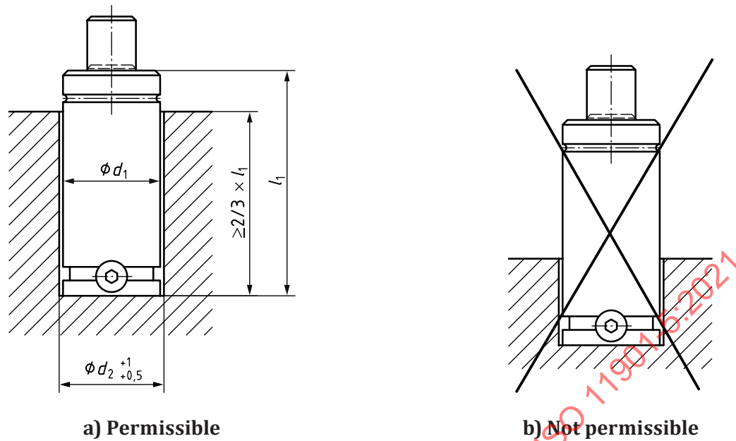
Figure A.15 — Mounting – inserted loosely in the hole
