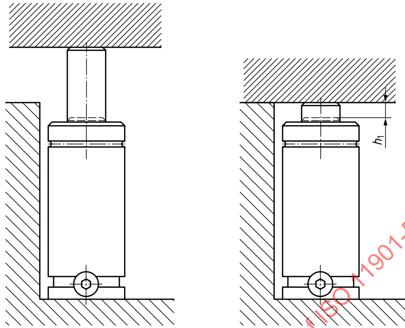
Figure A.6 — Permissible – operating at maximum working stroke
