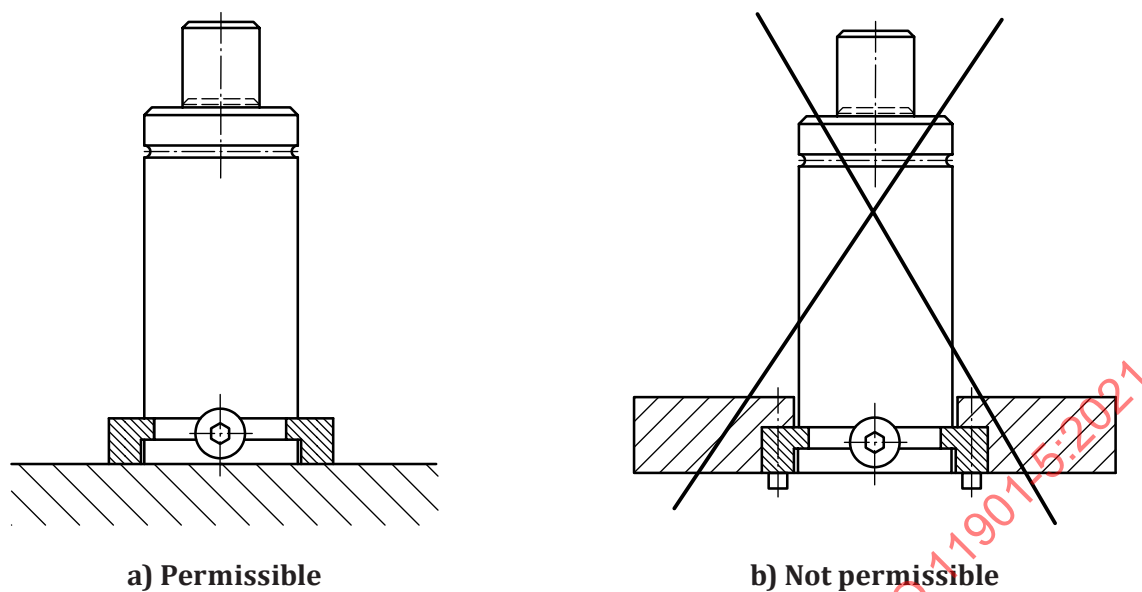
Figure A.10 — Two-part mounting clamps
