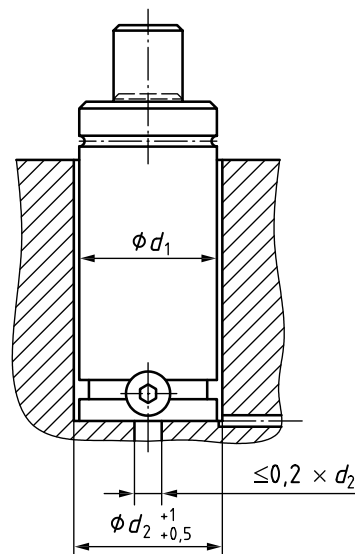
Figure A.16 — Installation in holes and pockets
