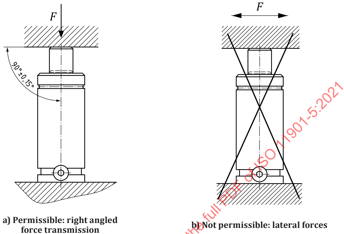
Figure A.5 — Force transmission
