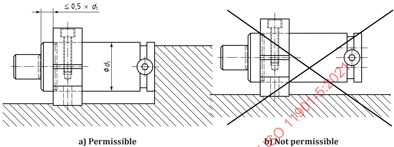
Figure A.12 — Clamping flange mounting
