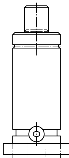
Figure A.13 — Mounting - bolted to the base
