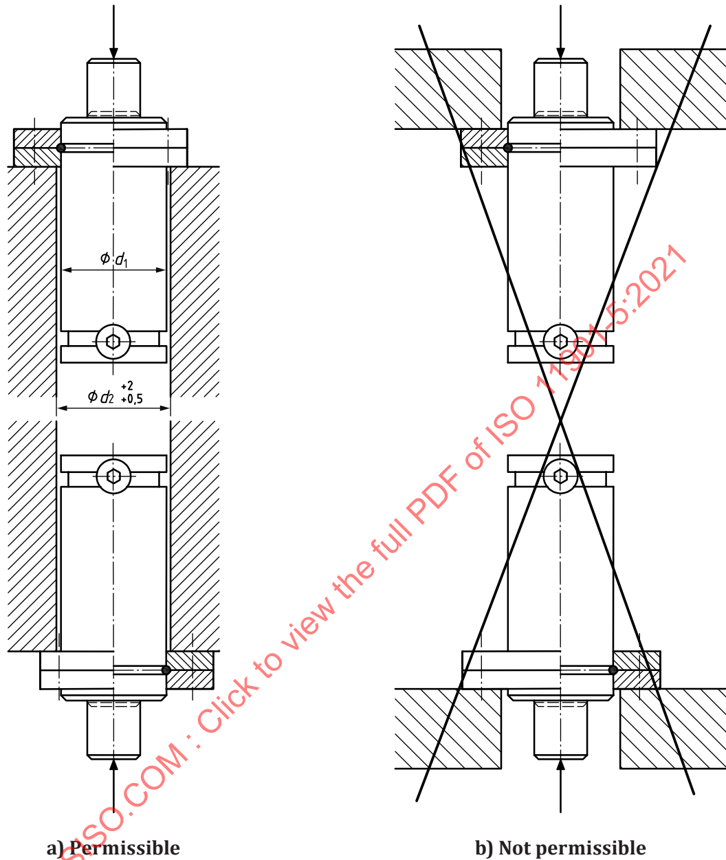
Figure A.9 — Lapped flange mounting
