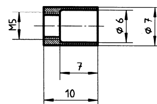
d) Flame stabilizer
