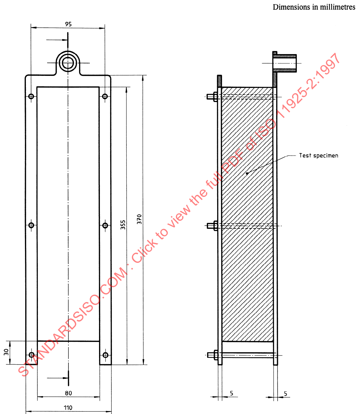
Figure 3 — Specimen holder
