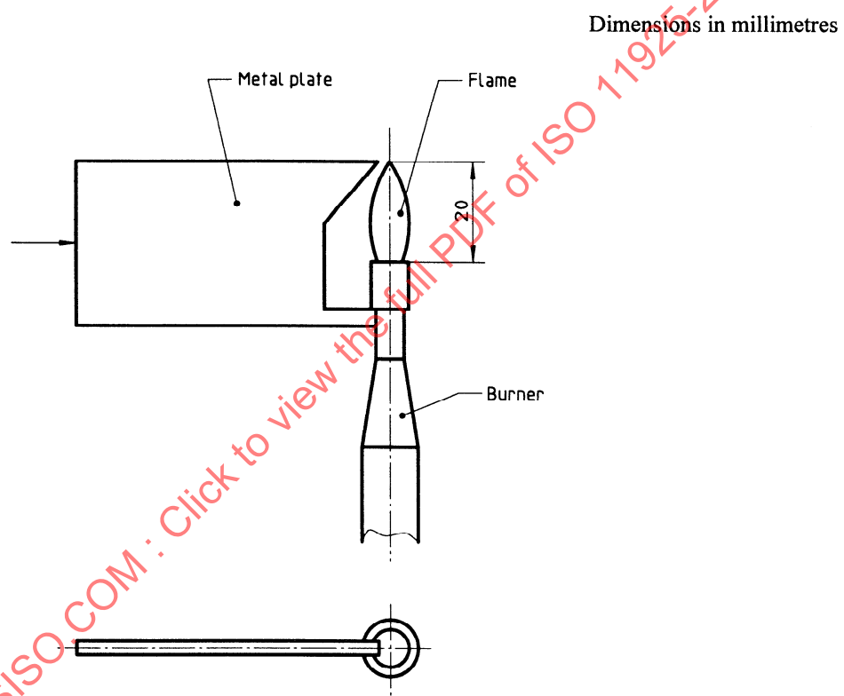
Figure 5 — Flame height measuring device
