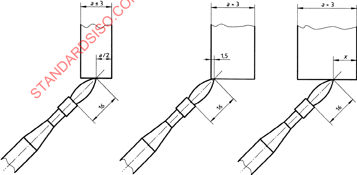
Figure 8 — Flame impingement points for one-layered products
