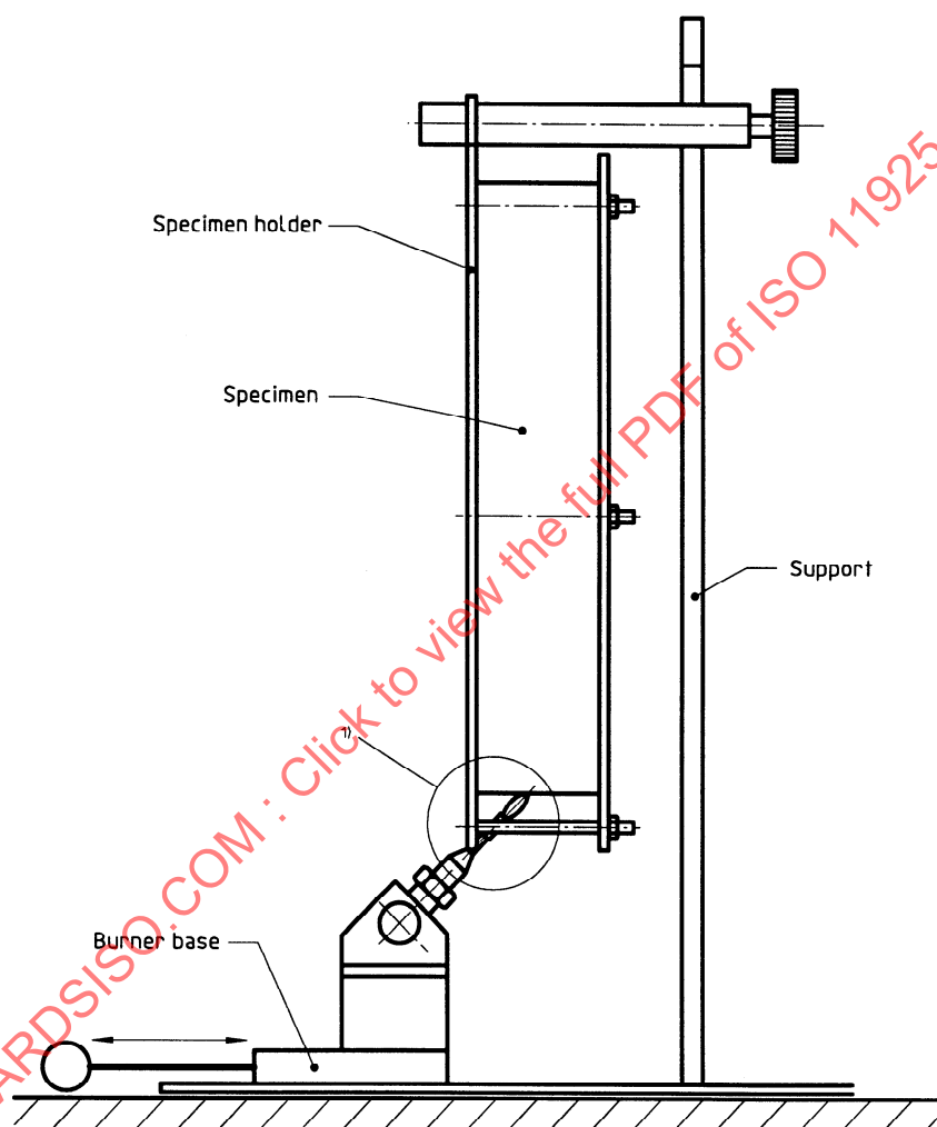
Figure 4 — Typical support and burner positioning (side view)
