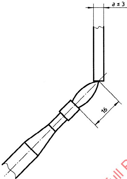
Figure 7 — Flame impingement points for one-layered products less than 3 mm thick
