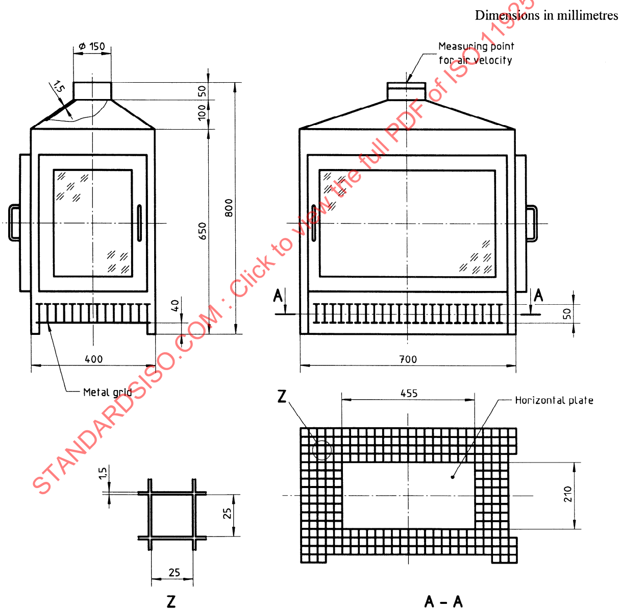
Figure 1 — Combustion chamber
