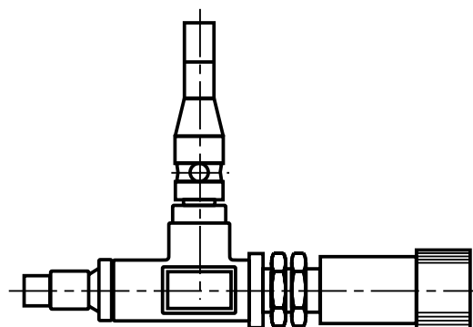
Figure 2 d) Flame stabilizer
