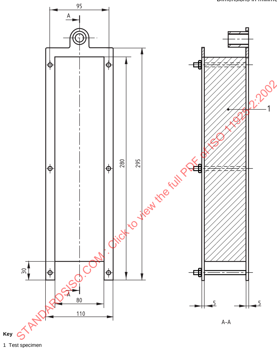
Figure 3 — Typical specimen holder
