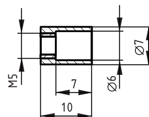
Figure 2 b) Gas jet
