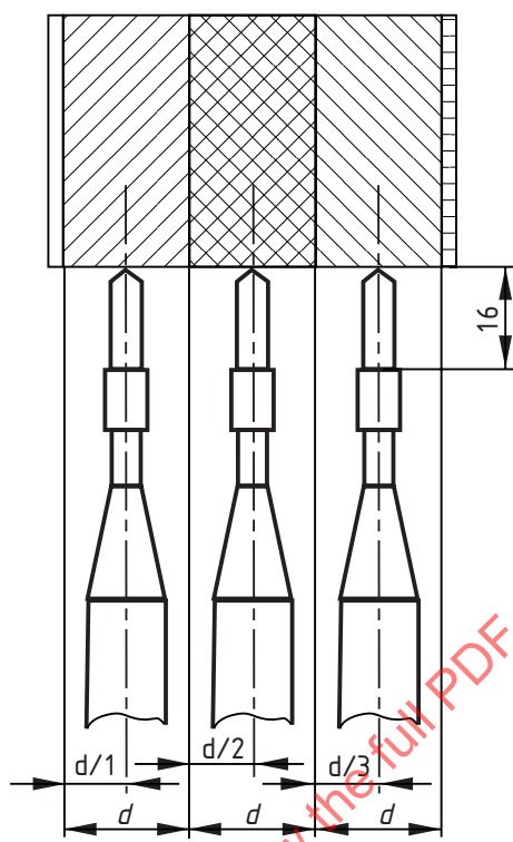
Figure 7 — Flame impingement points for additional set of tests for multilayer specimens greater than 10 mm thick
