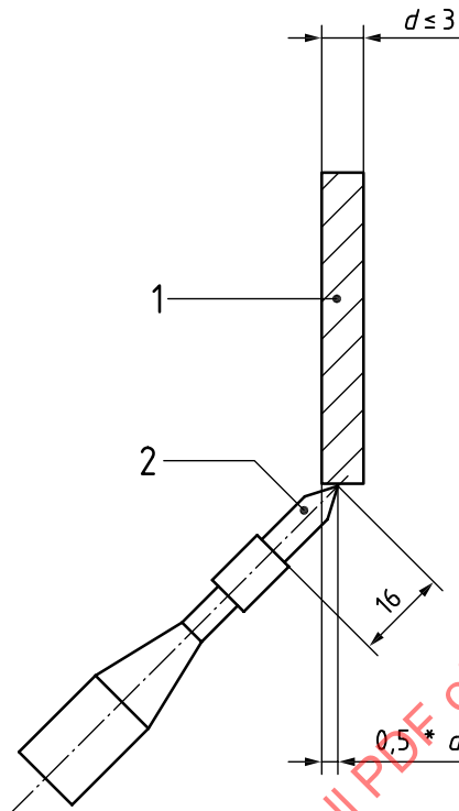
a) Flame impingement point for products less than or equal to 3 mm thick
