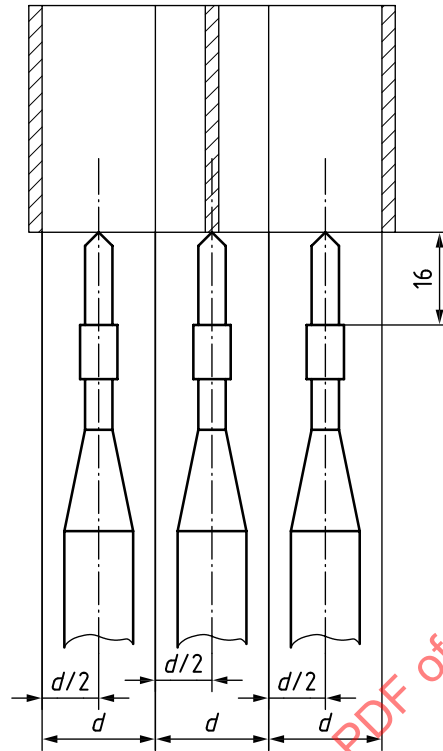
c) Flame impingement points for additional set of tests for multi-layer specimens greater than 10 mm thick with single layers greater than 3 mm thick
