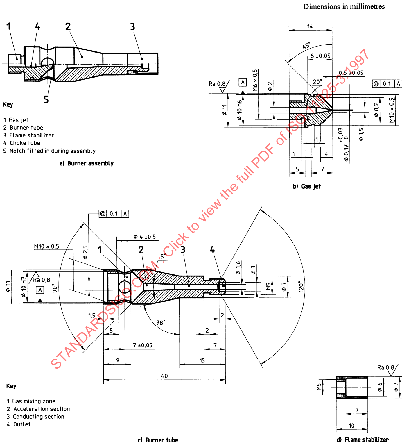
Figure 1 — Gas burner
