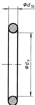
Figure 3 — O-ring
