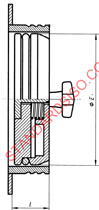
c) Cross-section with threaded knob
