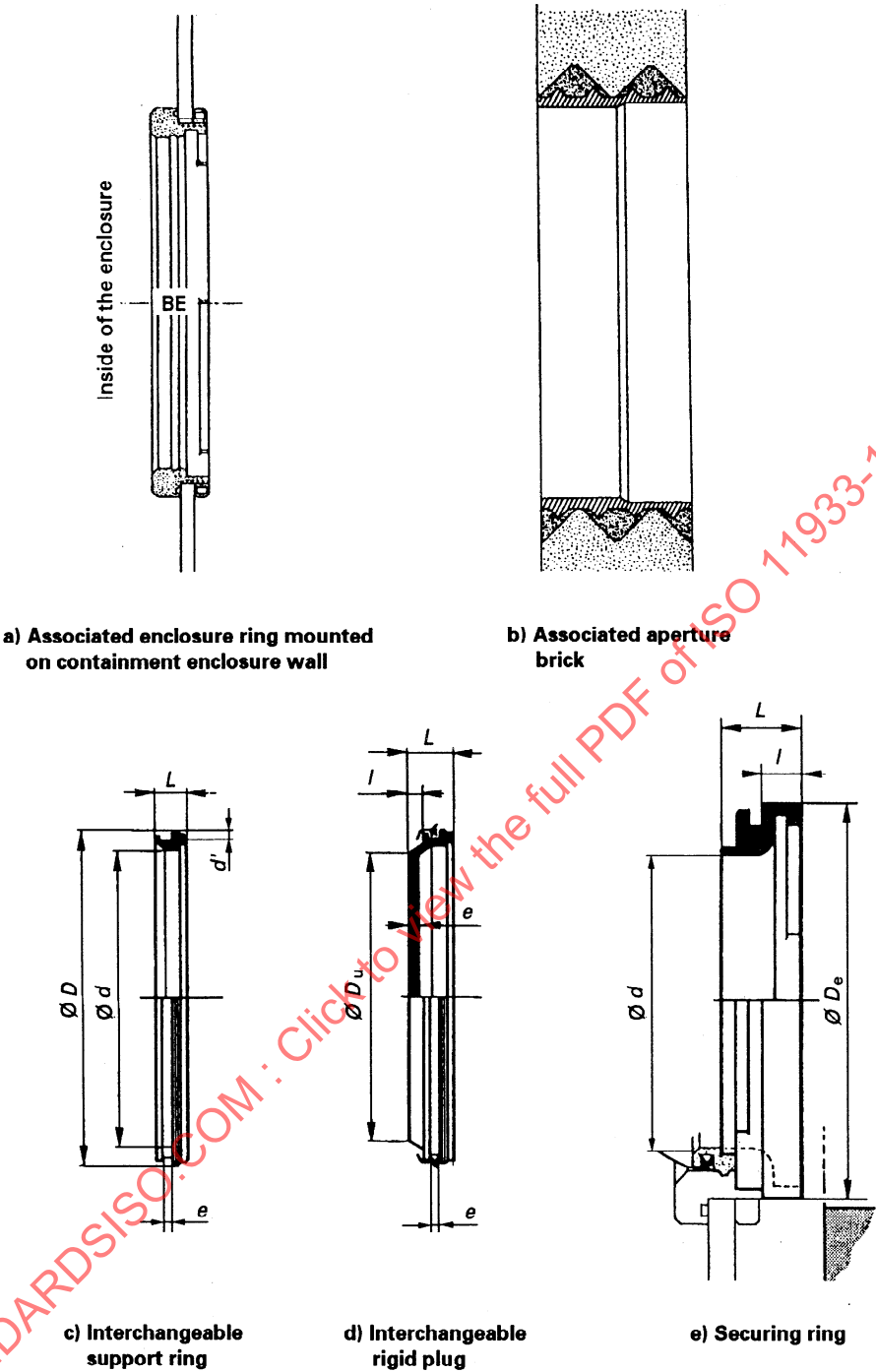
Figure 28 - Type 1 interchangeable units with associated units
