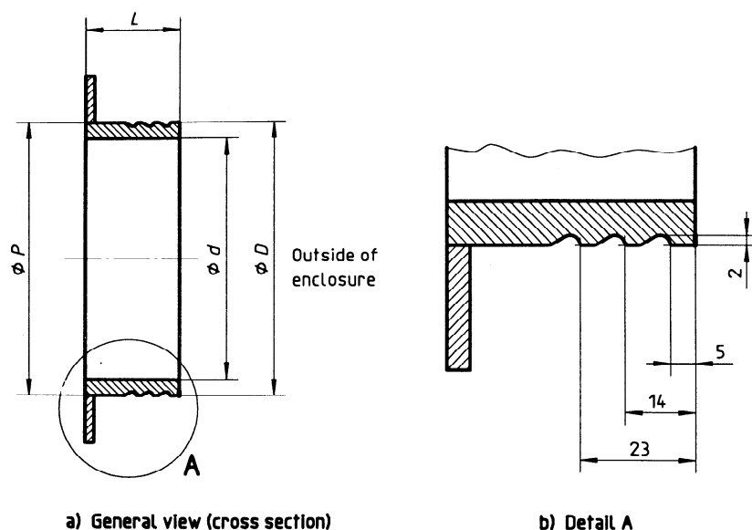
Figure 24 - Type 3 enclosure rings
