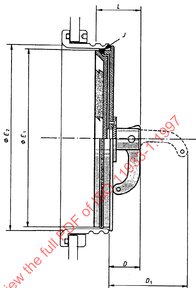
b) Cross-section with lever and additional shielding
