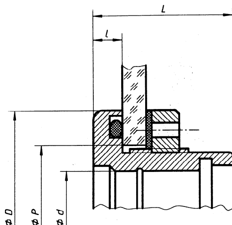
Figure 22 - Dimensions of type 2 enclosure rings
