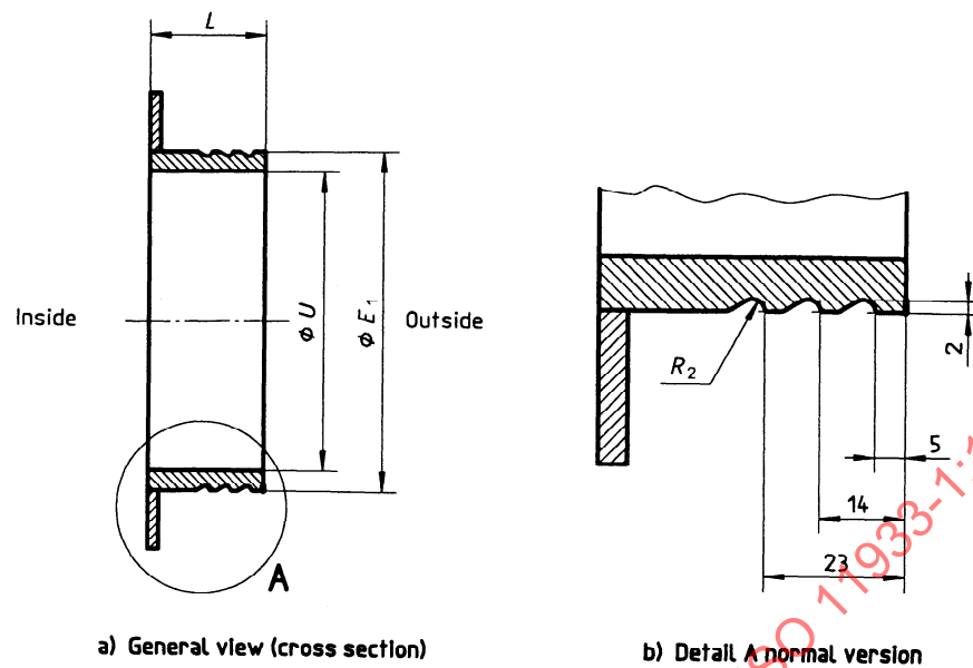
Figure 8 - Example and dimensions of bonded or welded glove/bag ports having three external grooves
