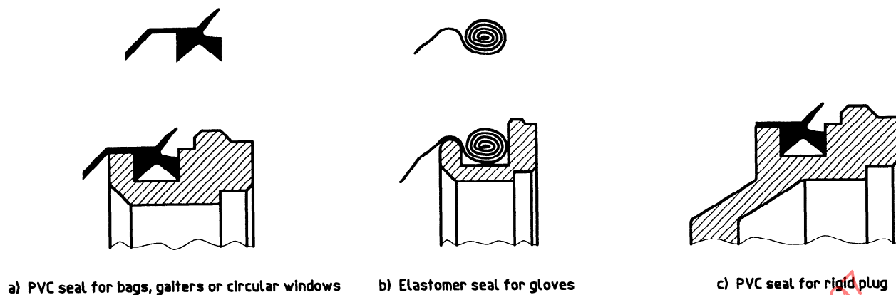
Figure 26 - Seals and assembly of seals
