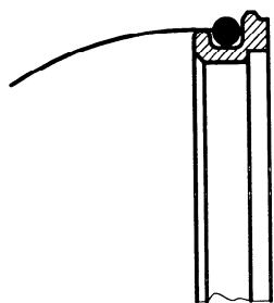
b1) Support rings equipped with: glove (or tong gaiter) made of elastomer
