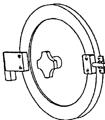
a) View from inside containment enclosure
