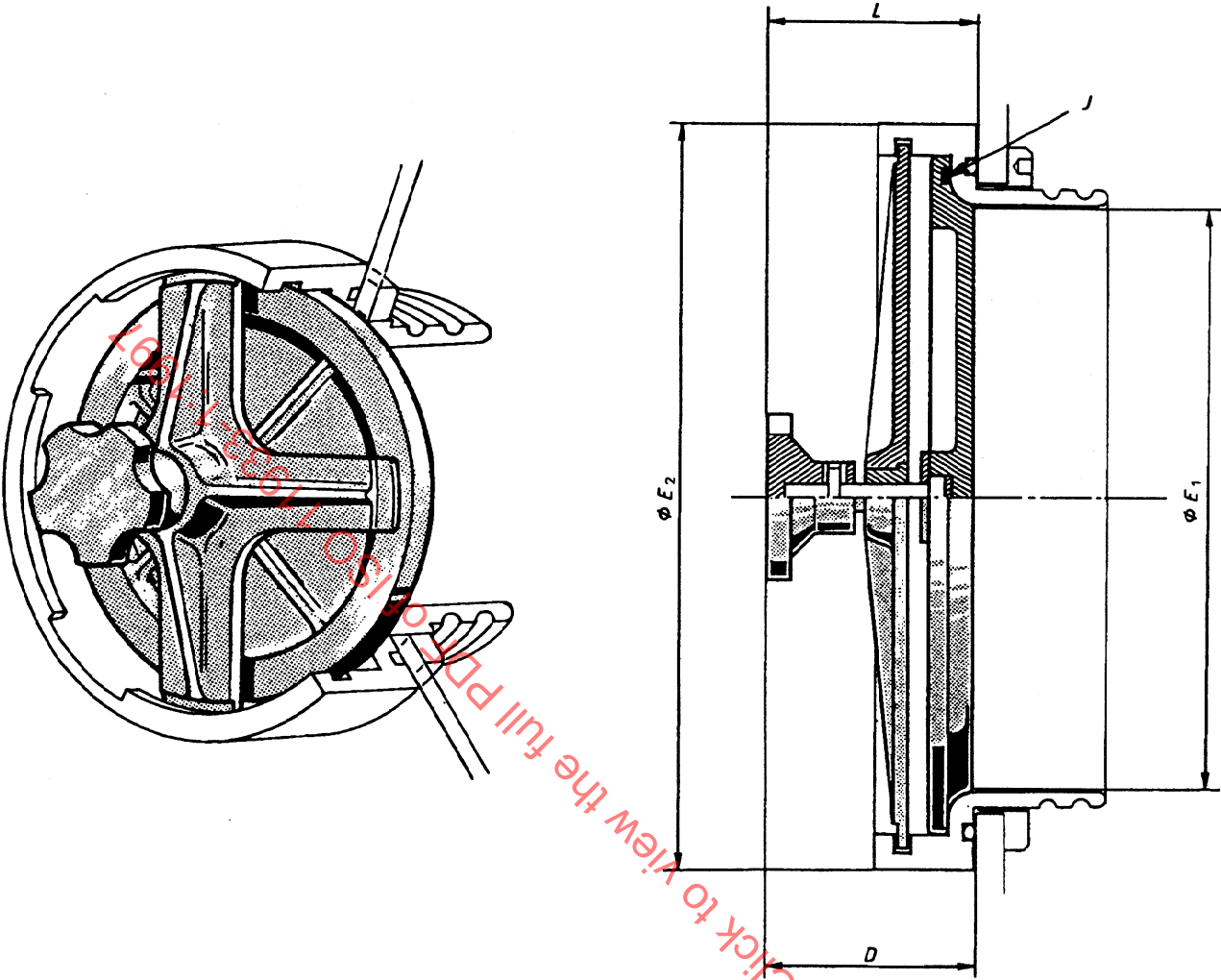
a) View from inside containment enclosure
