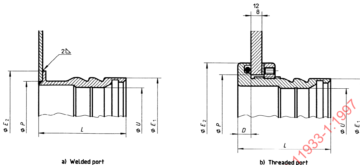
Figure 10 - Example and dimensions of glove/bag port which can accept two types of gloves/bags either directly on external grooves or with an ejectable support ring
