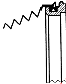
b3) Support rings equipped with: protective manipulator gaiter (or tong gaiter) made of PVC
