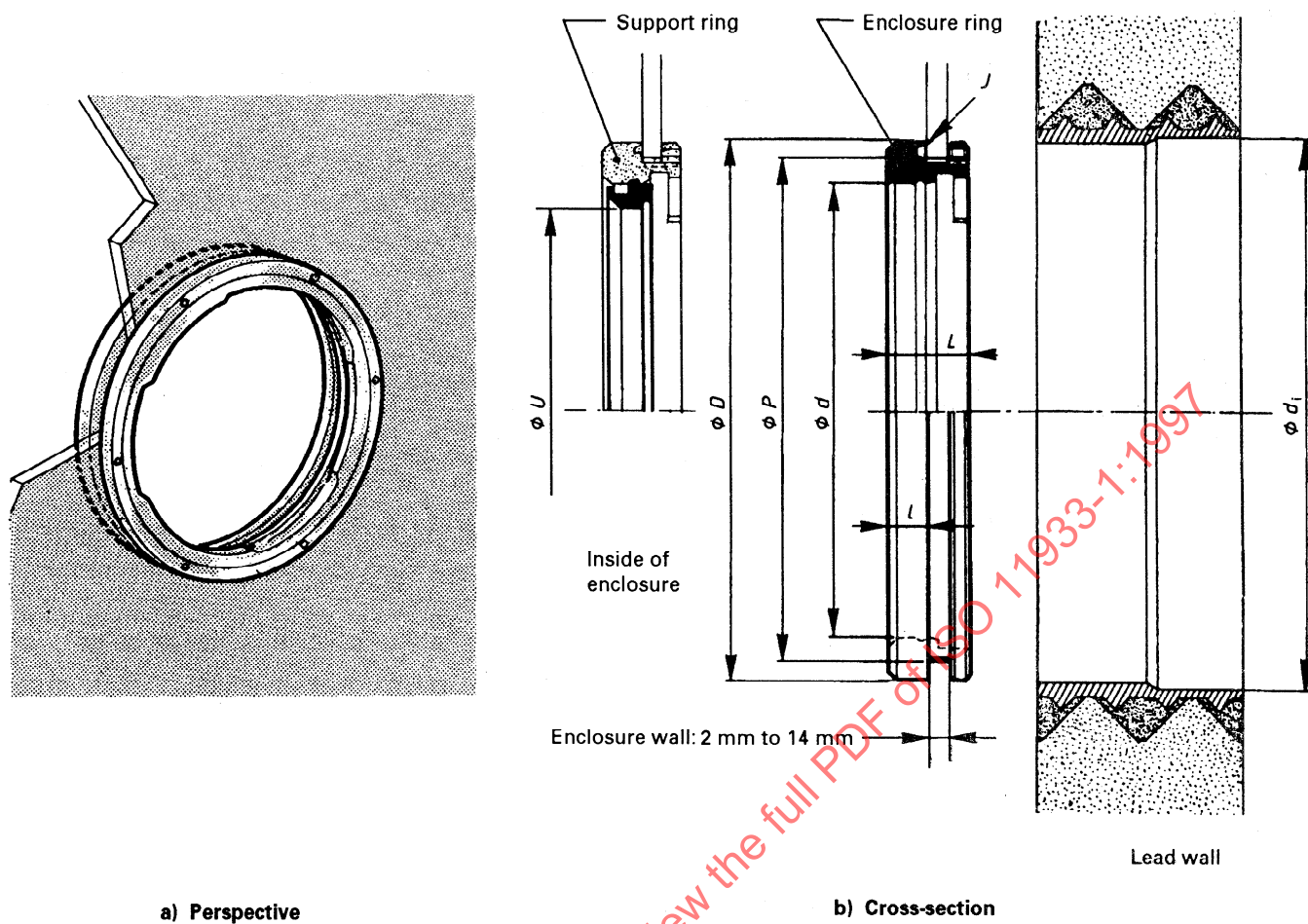
Figure 20 Type 1 enclosure rings
