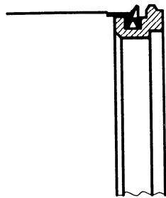
b2) Support rings equipped with: welded bag
