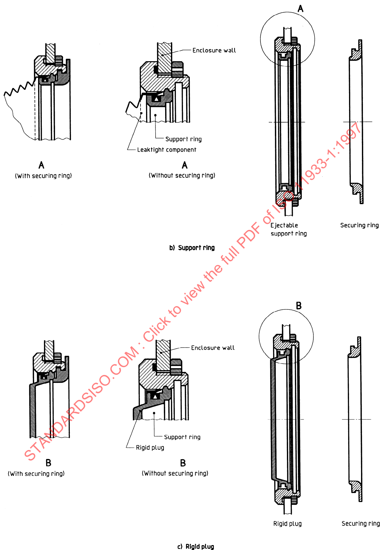
Figure 27 - Assembly of type 1 interchangeable units
