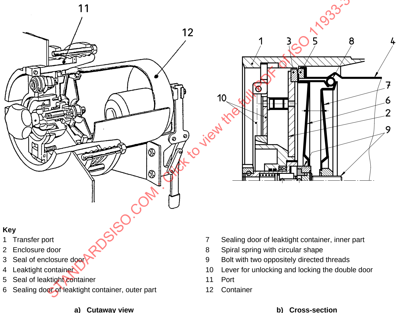
Figure 17 — Type 2 double door transfer system
