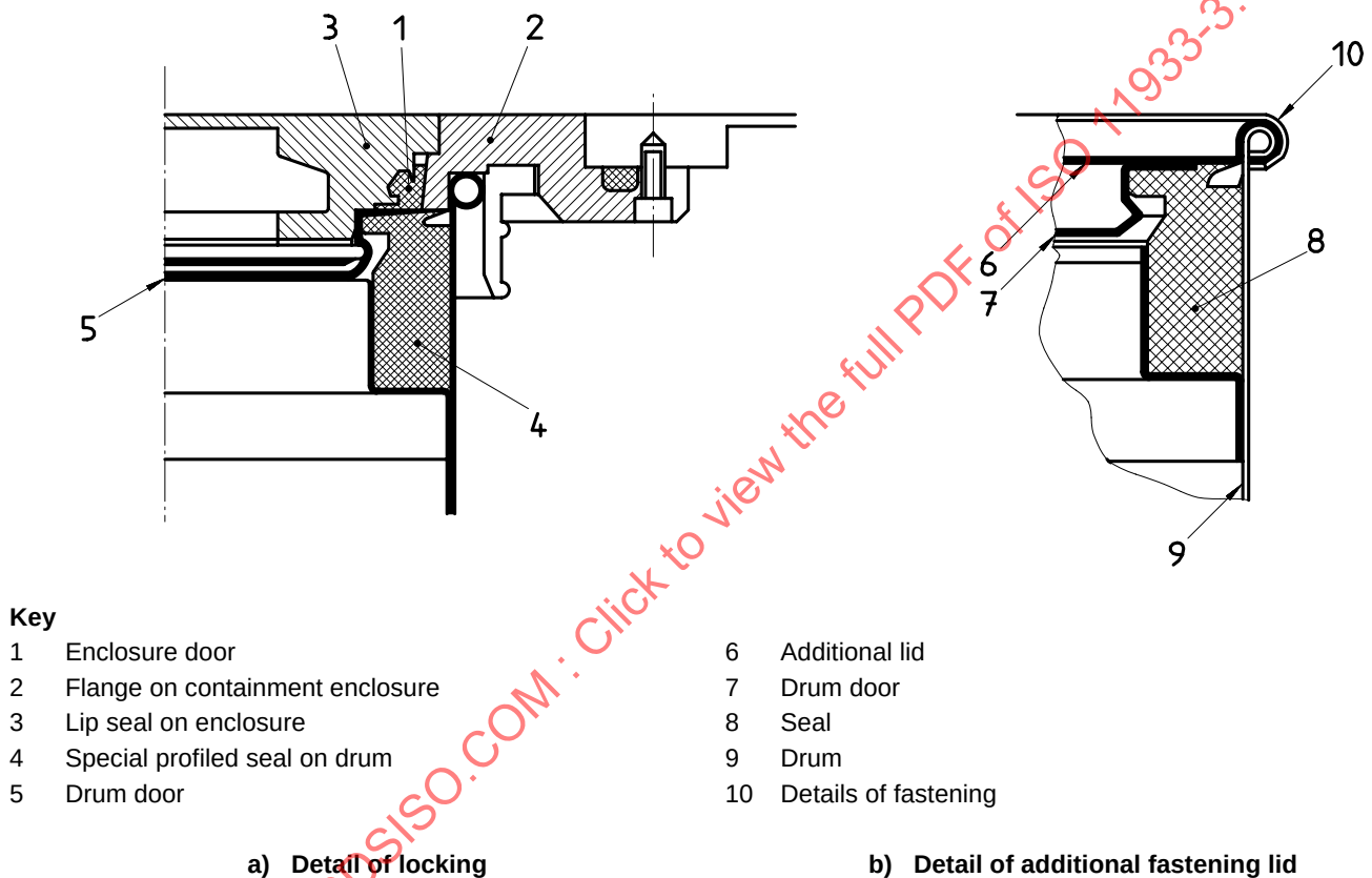
Figure 23 — Type 1 leaktight connection for waste drums
