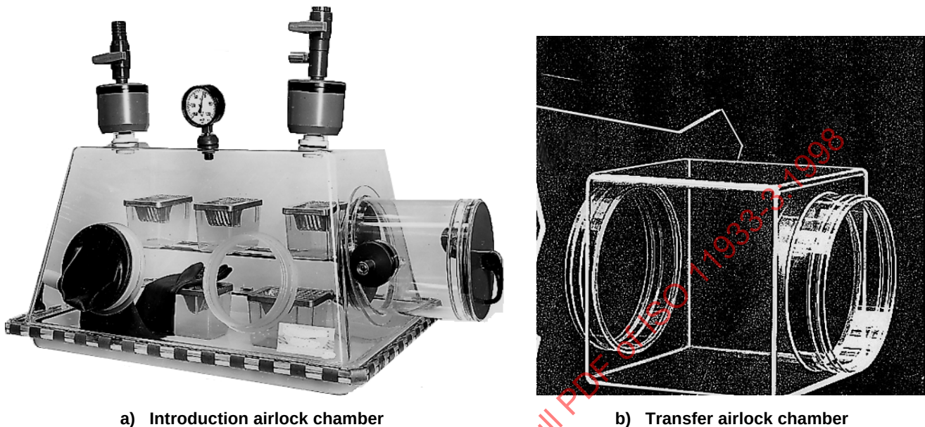
Figure 6 — General view of an airlock chamber
