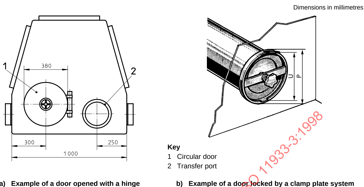
Figure 4 — Standard dimensions of circular plain doors
