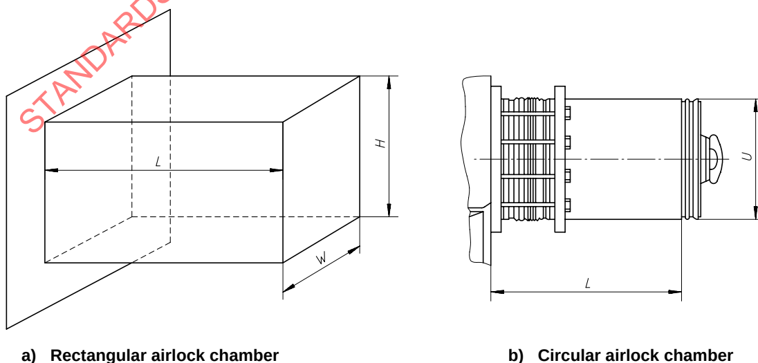
Figure 10 — Dimensions of introduction airlock chambers
