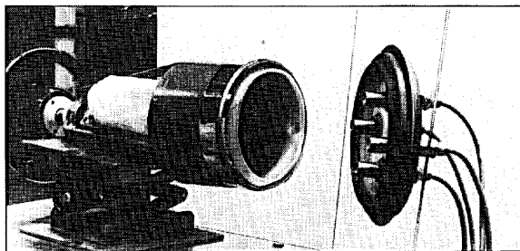
a) Connection of the ejecting device on the ejectable rigid plug equipped with wall penetrations
